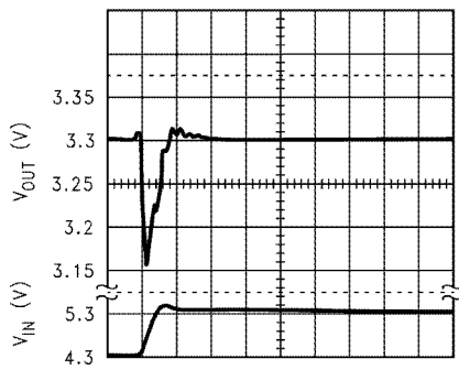
Line Transient Response ( I_{OUT} = 3.0A )
