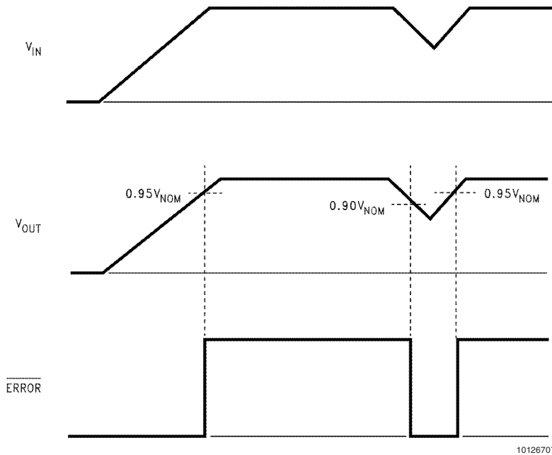
FIGURE 1. \overline{\text{Error}} Flag Operation
