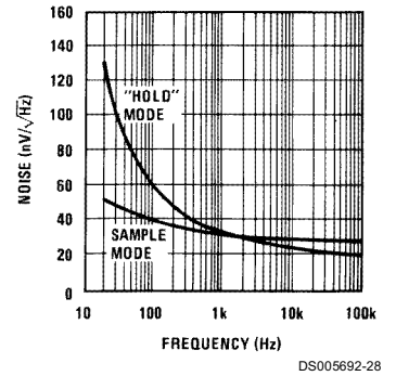
Output Noise
