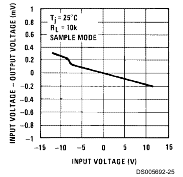
Gain Error
