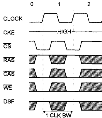
Timing Diagram to Illustrate t BWC
