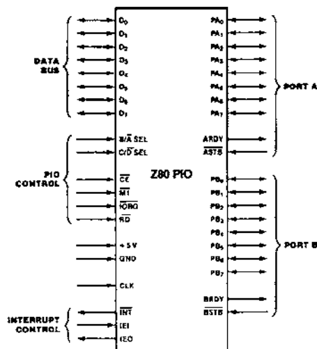
Figure 1. Pin Functions
