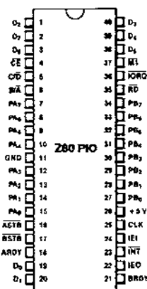
Figure 2a. 40-pin Dual-in-Line Package (DIP), Pin Assignments
