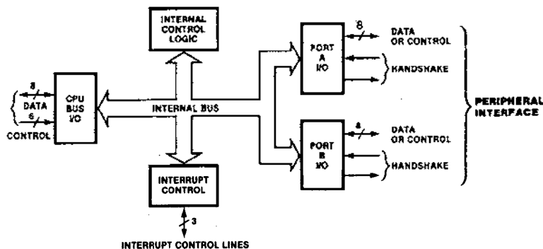
Figure 4. Block Diagram
