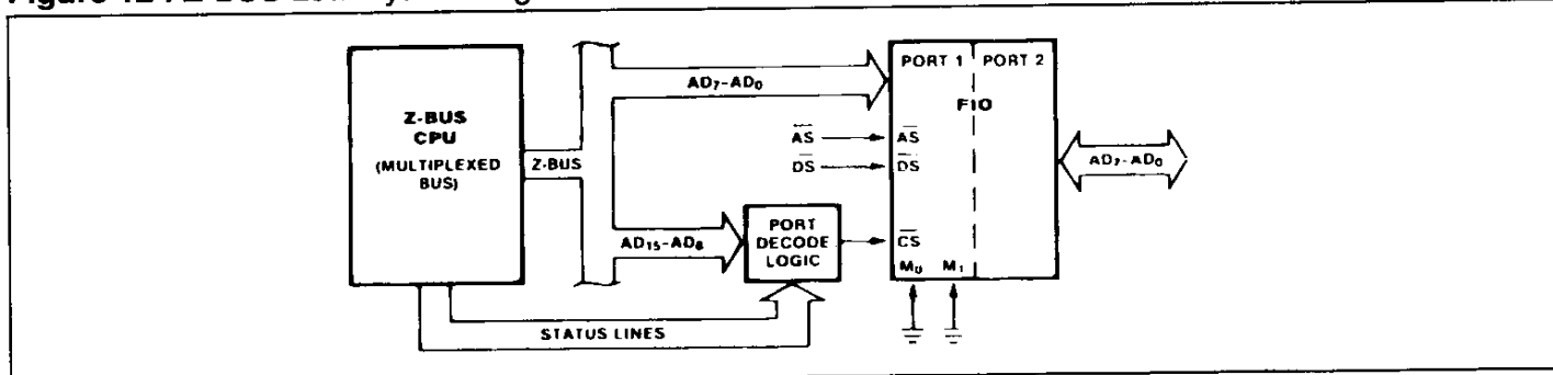
Figure 12 : Z-BUS Low-Byte Configuration.
