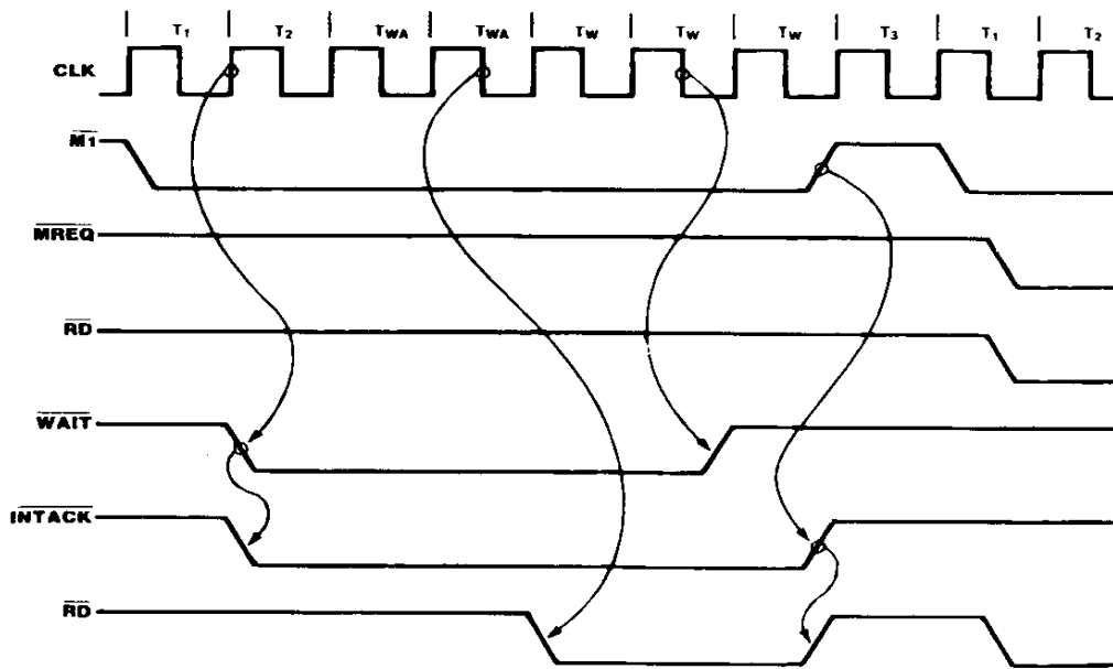
Figure 44 : Z80 Interrupt Acknowledge Timing.
