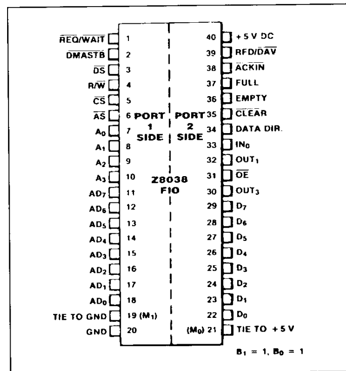
Figure 63 : Z-BUS-High-Byte to 2-Wire Handshake.
