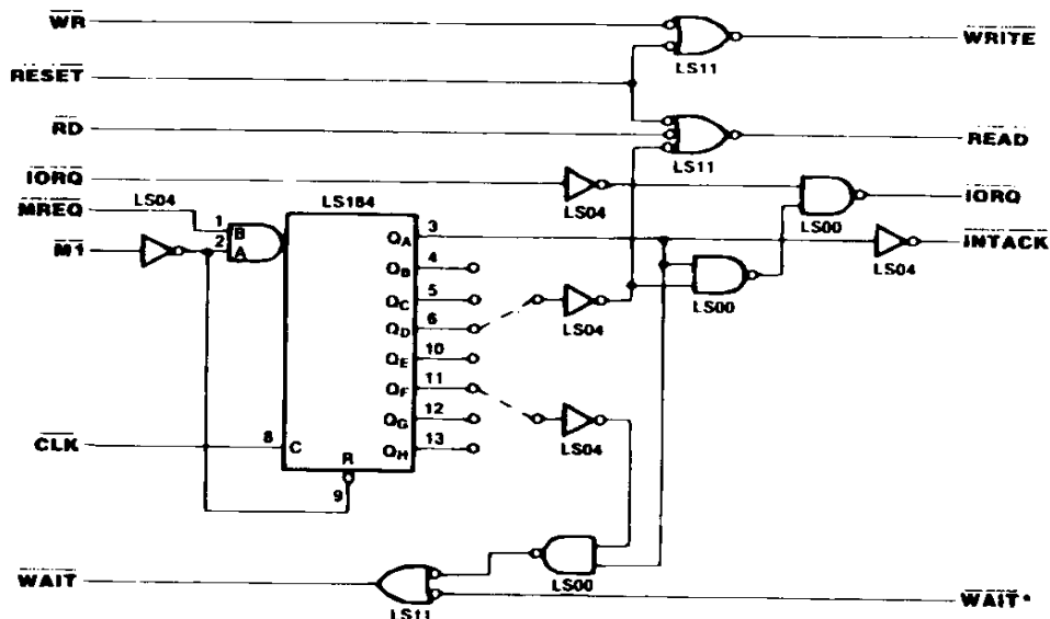
Figure 45 : External Logic Interfacing the Z80 to 8500 Series Peripherals.
