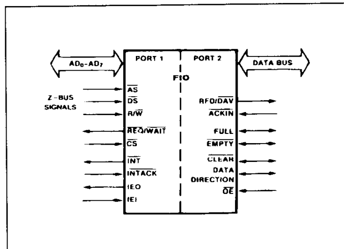
Figure 18 : Wire Handshake I/O Configuration.
