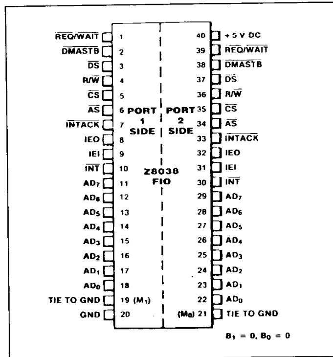
Figure 56 : Z-BUS-Low-Byte to Z-BUS-Low-Byte.
