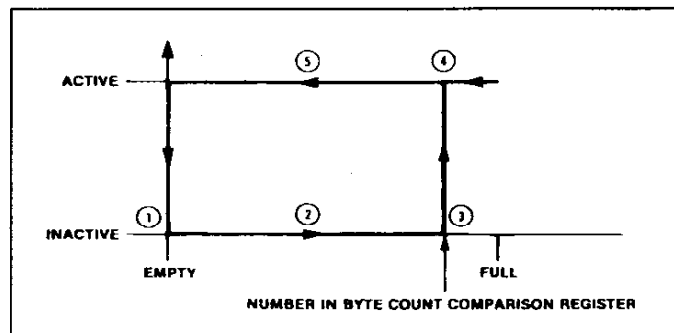
Figure 30 : Request Hysteresis Diagram : Read from FIO.
