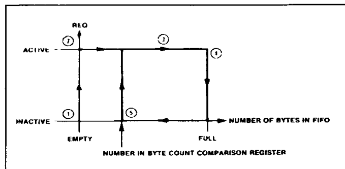
Figure 29 : Request Hysteresis Diagram : Write to FIO.
