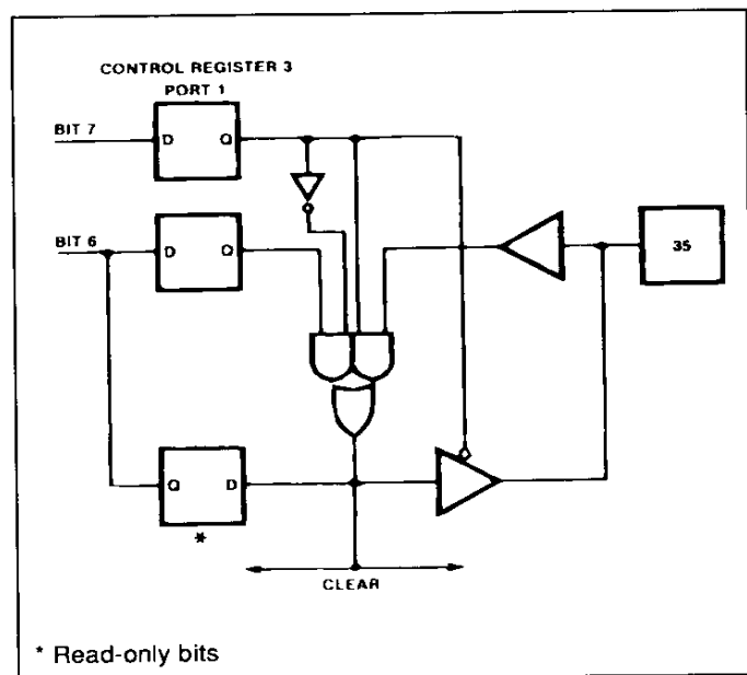
Figure 39 : CLEAR : CPU-to-I/O Operation.
