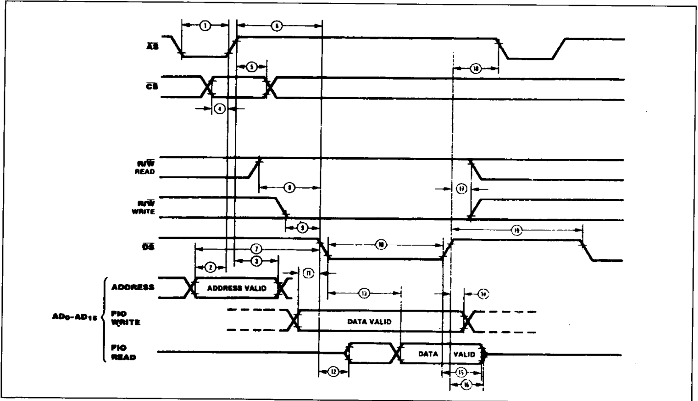
Figure 81 : Z-BUS CPU Interface Timing.
