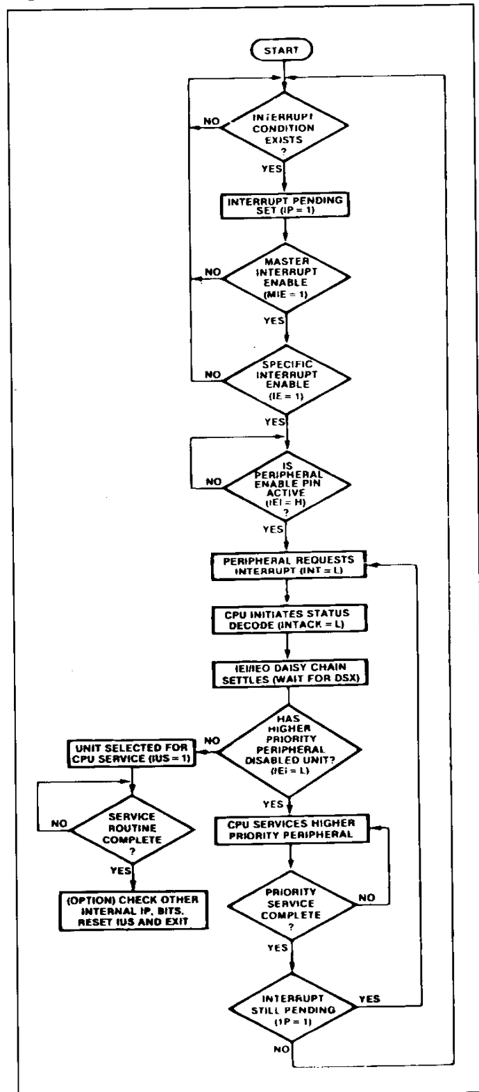
Figure 31 : Interrupt Flowchart.
