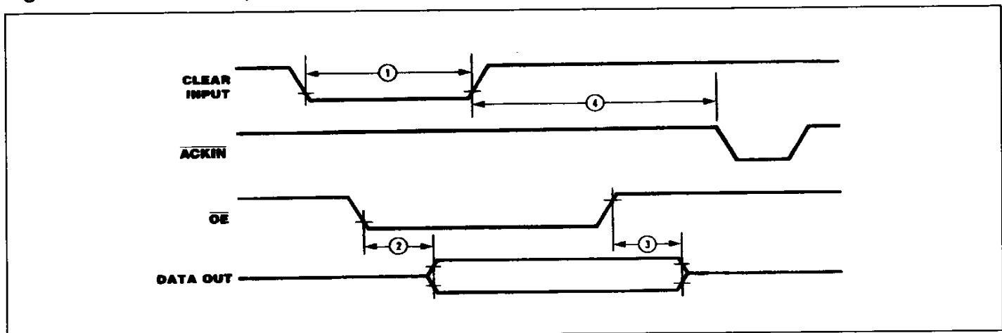
Figure 92 : Port 2 Side Operation.
