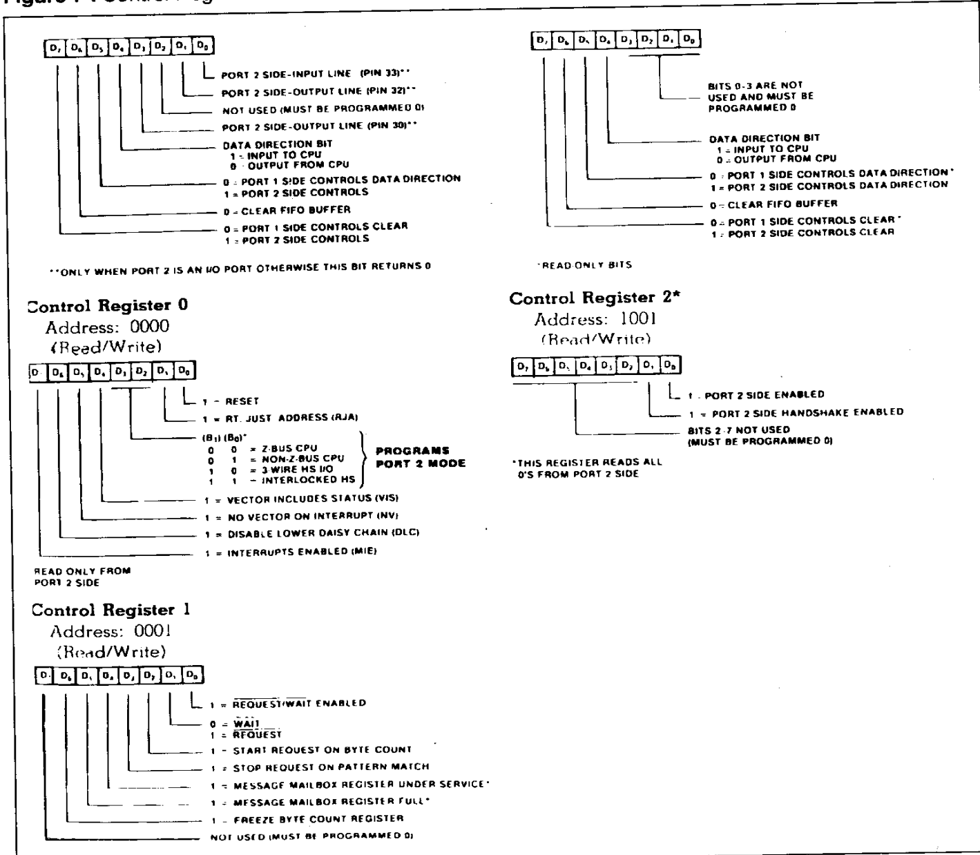
Figure 7 : Control Registers 0-3.
