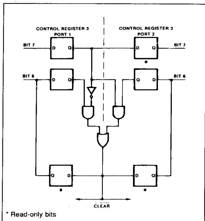
Figure 37 : CLEAR : CPU-to-CPU Operation.
