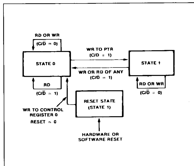
Figure 17 : Register Access State Diagram.
