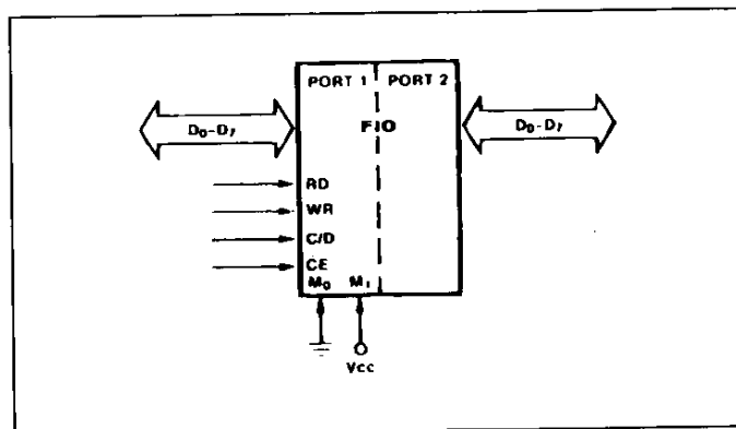
Figure 15 : Non-Z-BUS (nonmultiplexed) Microprocessor Configuration.
