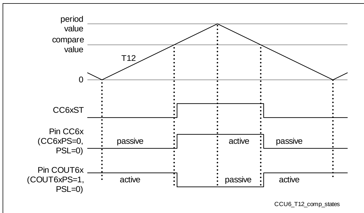
Figure 14-4 Compare States of Timer T12
