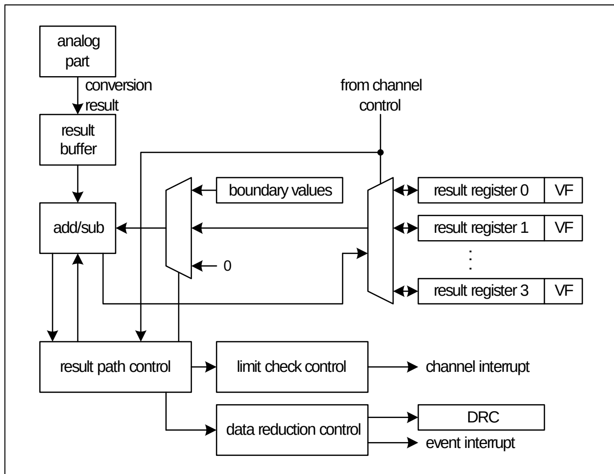
Figure 16-8 Result Path
