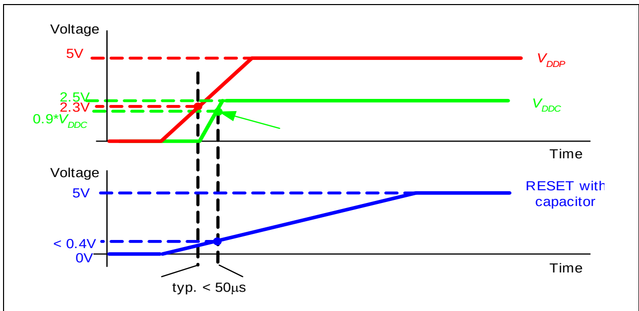
Figure 7-3 V_{DD} , V_{DDC} and V_{RESET} during Power-on Reset
