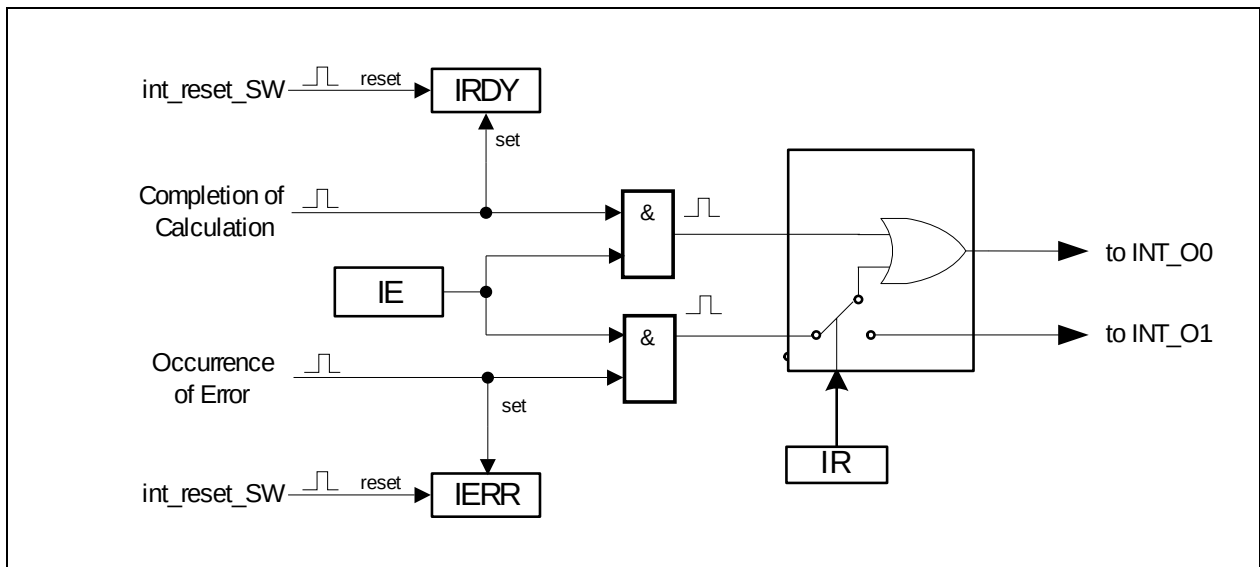
Figure 10-2 Interrupt Generation
