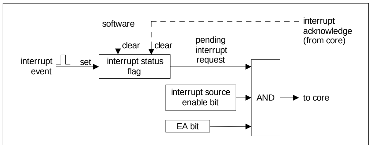
Figure 5-7 Interrupt Structure 1
