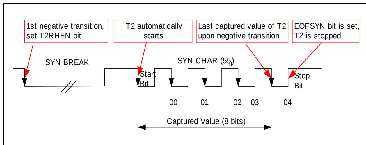
Figure 18-2 LIN Auto Baud Rate Detection for Header LIN Frame
