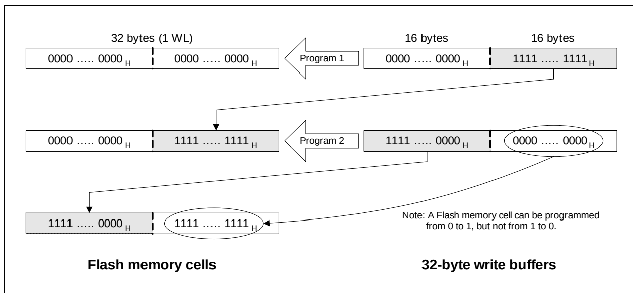
Figure 4-7 D-Flash Program
