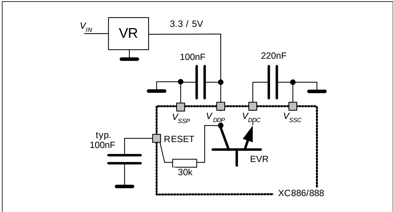
Figure 7-2 Reset Circuitry
