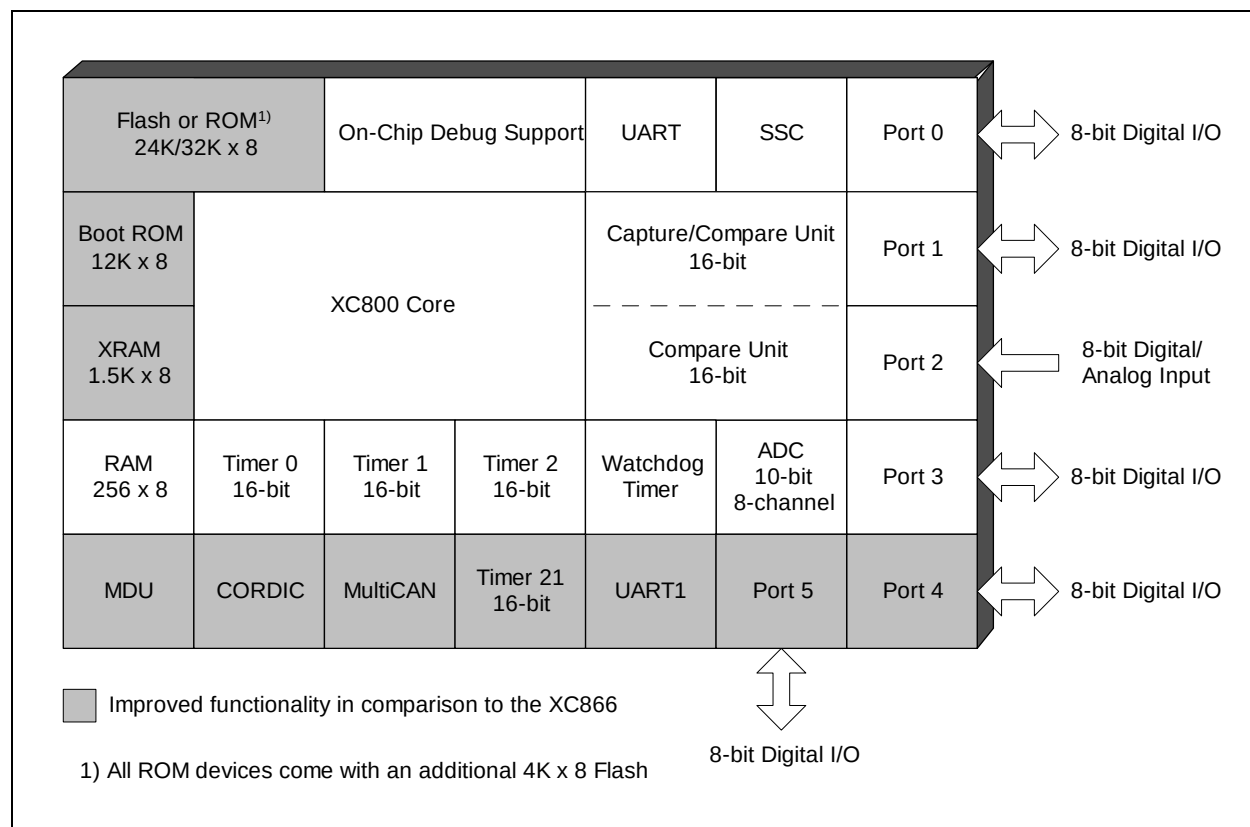
Figure 1-1 XC886/888 Functional Units
