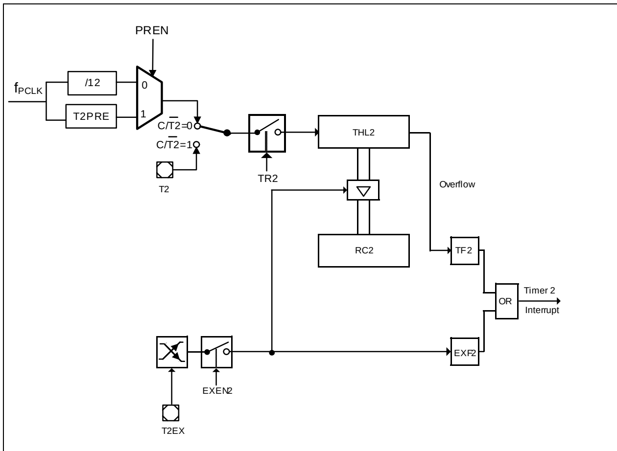
Figure 13-7 Capture Mode
