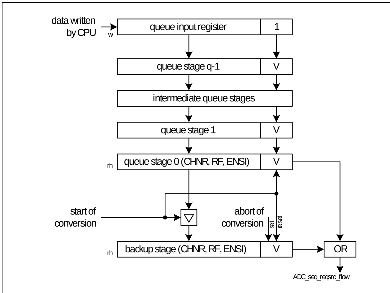
Figure 16-5 Multi-Stage Queue
