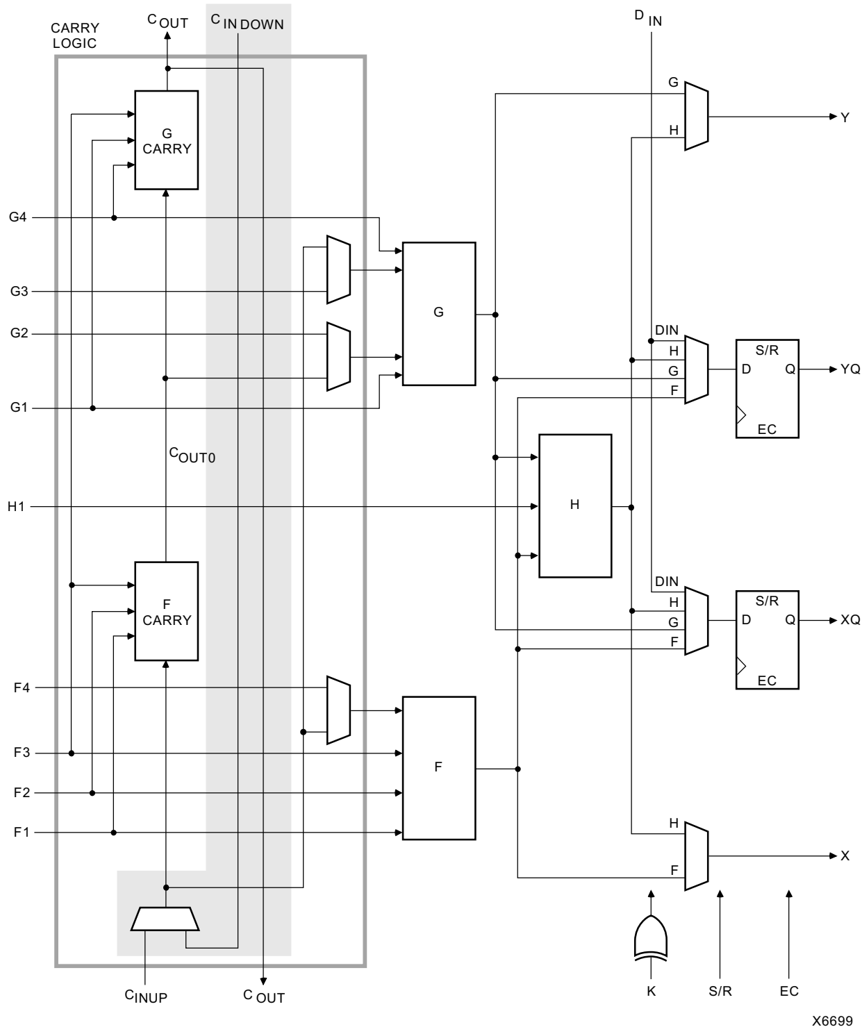
Figure 13: Fast Carry Logic in XC4000E CLB (shaded area not present in XC4000X)
