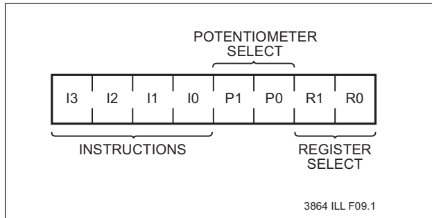
Figure 2. Instruction Byte Format
