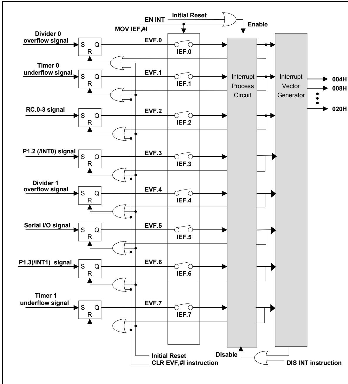
Figure 5-8 Interrupt event control diagram
