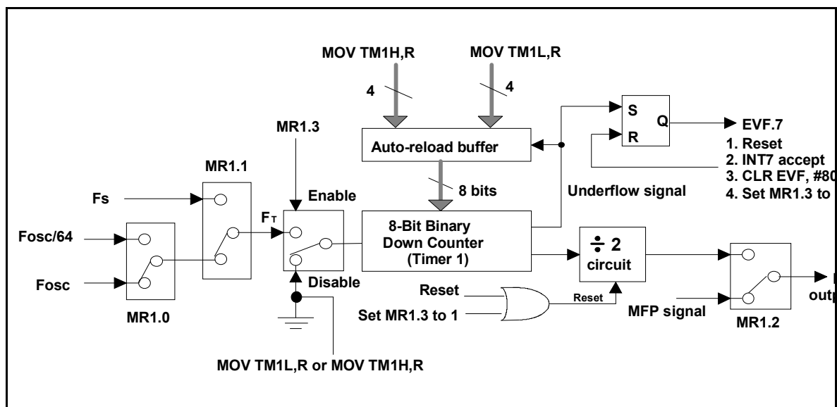
Figure 5-7 Organization of Timer 1
