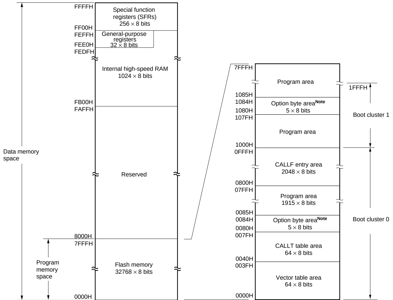
Figure 3-3. Memory Map ( \mu PD78F0114H)
