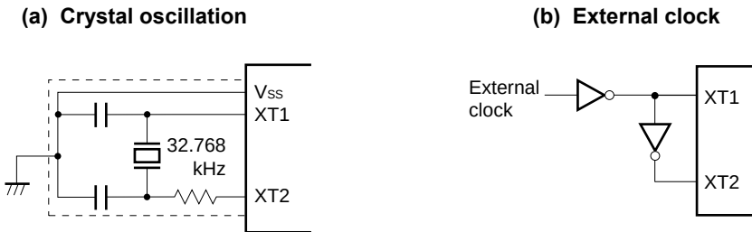
Figure 5-10. Examples of External Circuit of Subsystem Clock Oscillator
