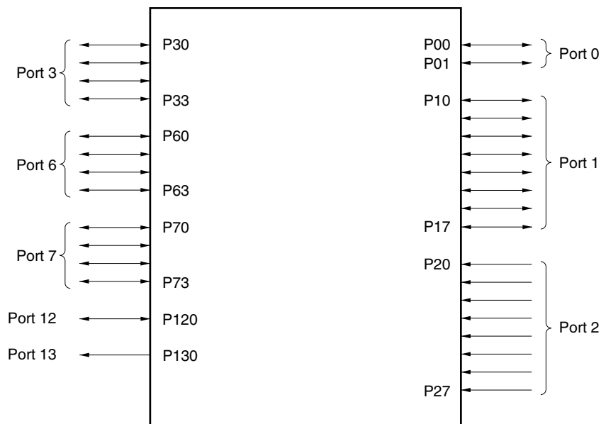
Figure 4-1. Port Types
