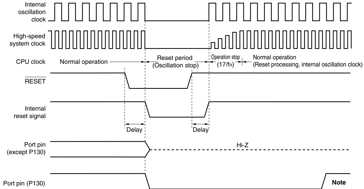
Figure 18-2. Timing of Reset by \overline{\text{RESET}} Input
