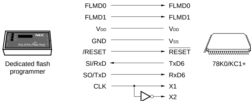
Figure 23-8. Communication with Dedicated Flash Programmer (UART6)
