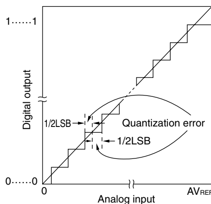
Figure 11-14. Quantization Error
