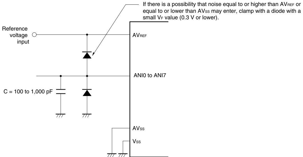
Figure 11-19. Analog Input Pin Connection
