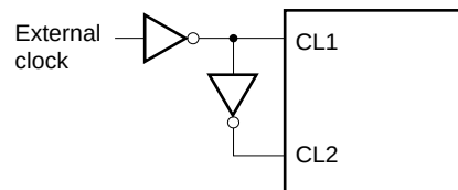
(b) External clock
