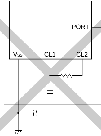
(b) Crossed signal line
