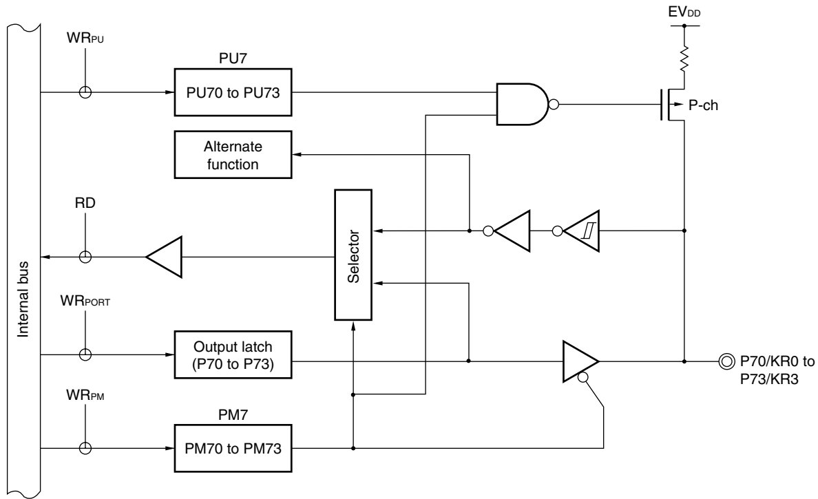
Figure 4-13. Block Diagram of P70 to P73
