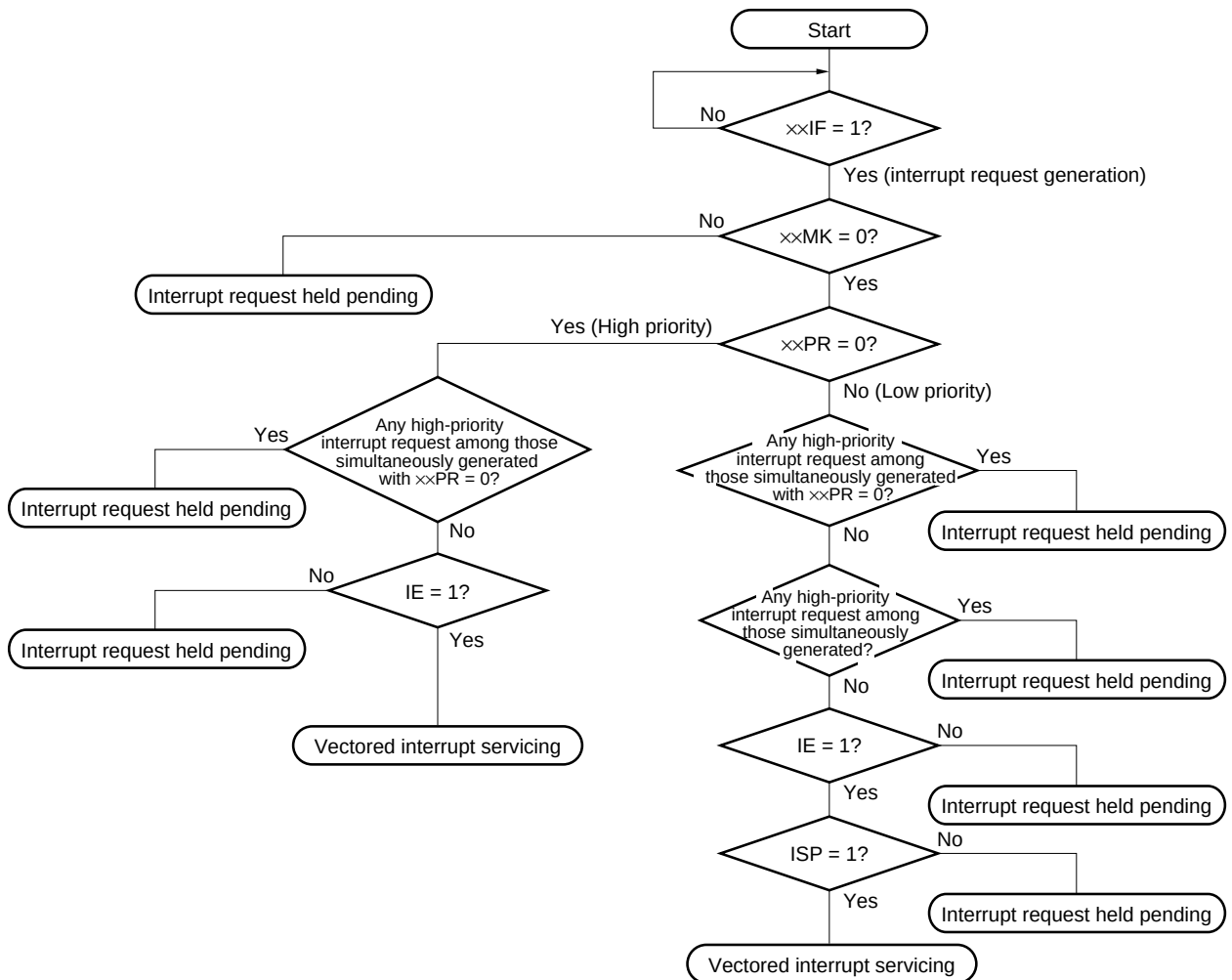
Figure 15-7. Interrupt Request Acknowledgment Processing Algorithm
