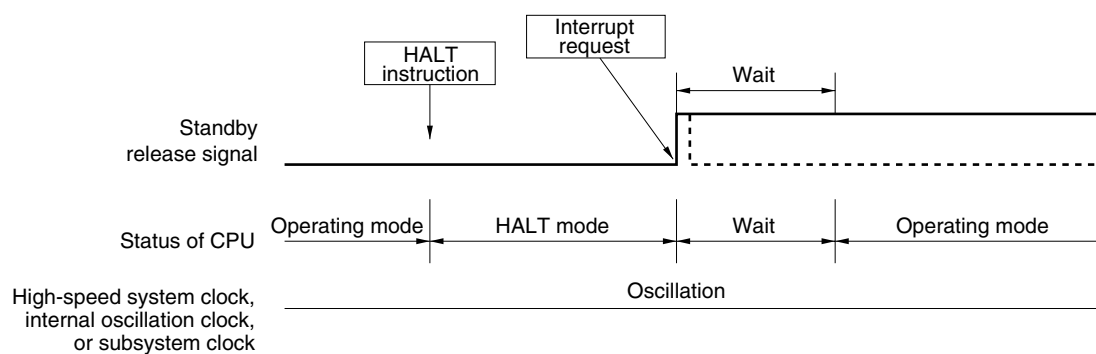
Figure 17-3. HALT Mode Release by Interrupt Request Generation
