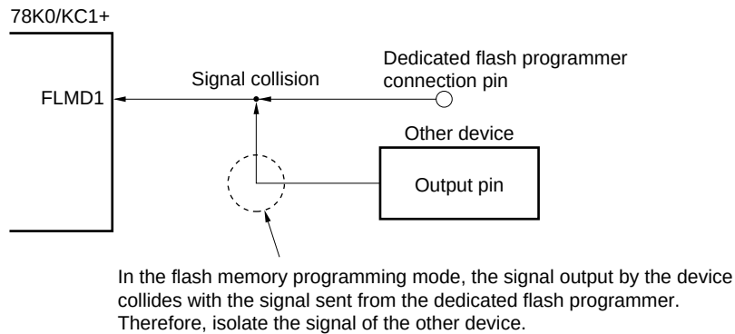
Figure 23-11. Signal Collision (Input Pin of Serial Interface)
