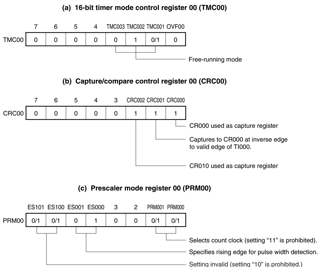
Figure 6-22. Control Register Settings for Pulse Width Measurement with Free-Running Counter and Two Capture Registers (with Rising Edge Specified)
