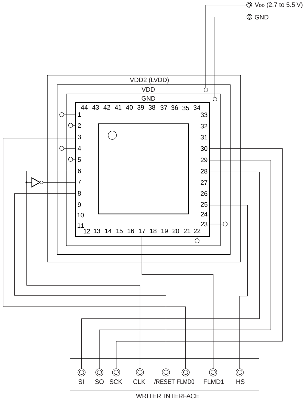
Figure 23-3. Example of Wiring Adapter for Flash Memory Writing in 3-Wire Serial I/O Mode (CSI10 + HS)
