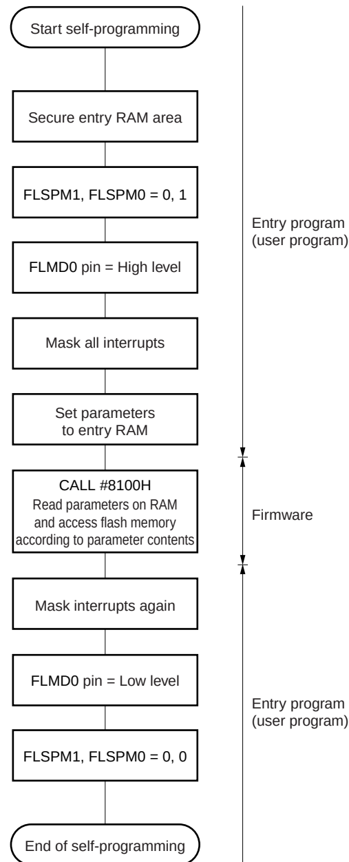
Figure 23-17. Self-Programming Procedure
