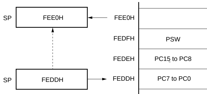
(c) RETI, RETB instructions (when SP = FEDDH)
