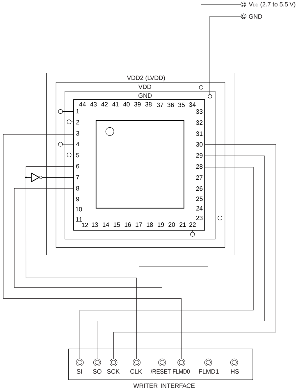
Figure 23-2. Example of Wiring Adapter for Flash Memory Writing in 3-Wire Serial I/O Mode (CS110)
