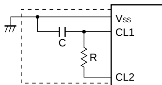
(a) RC oscillation
