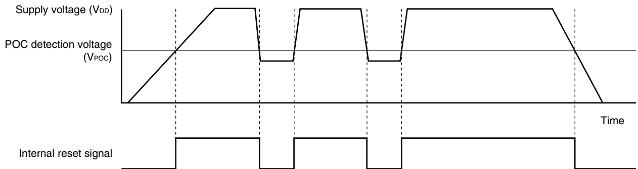
Figure 20-2. Timing of Internal Reset Signal Generation in Power-on-Clear Circuit
