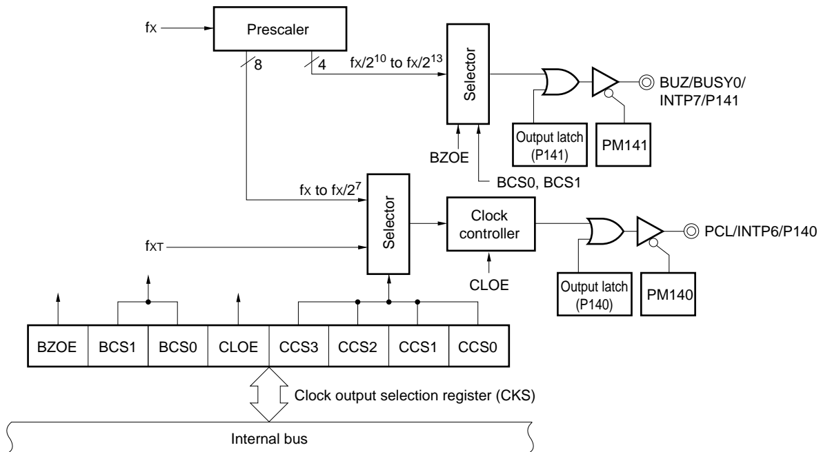
★ Figure 12-1. Block Diagram of Clock Output/Buzzer Output Controller
