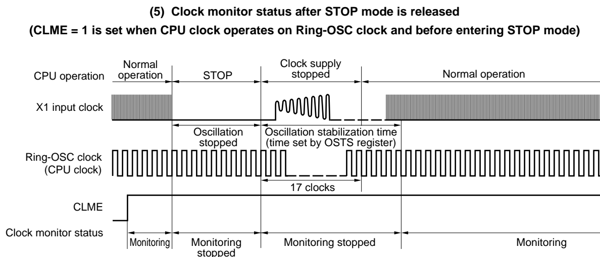
Figure 23-3. Timing of Clock Monitor (3/4)
