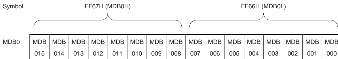
★ Figure 18-4. Format of Multiplication/Division Data Register B0 (MDB0)
