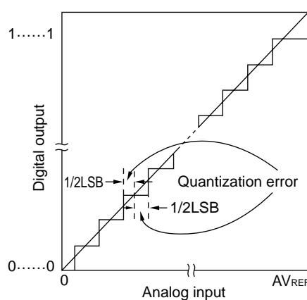
Figure 13-13. Quantization Error
