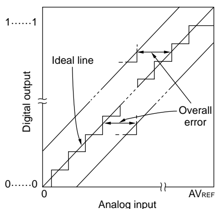
Figure 13-12. Overall Error
