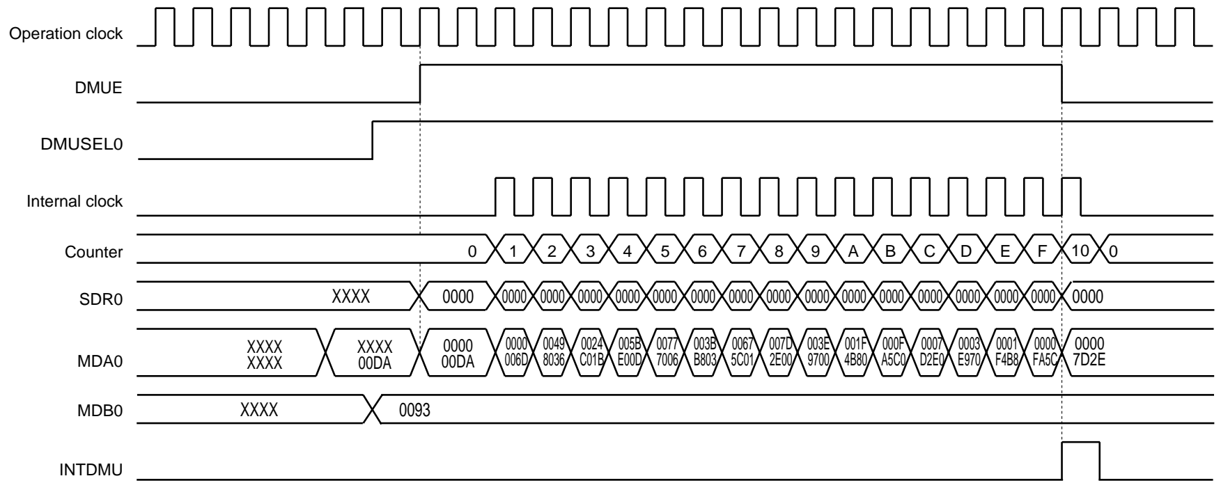
★Figure 18-6. Timing Chart of Multiplication Operation (00DAH × 0093H)
