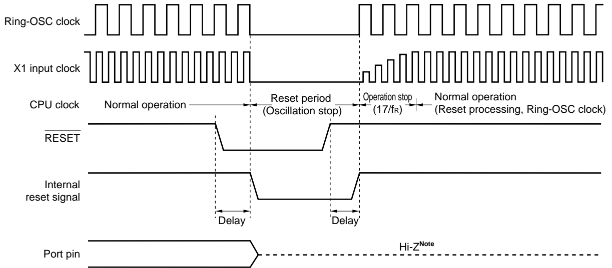
Figure 22-2. Timing of Reset by \overline{\text{RESET}} Input
