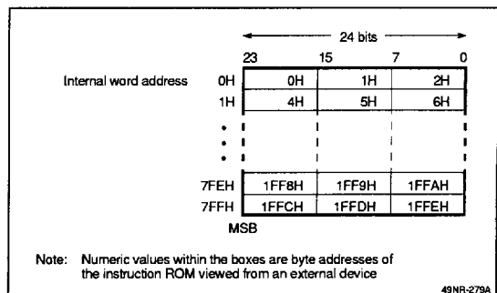
Figure 13. Instruction ROM
