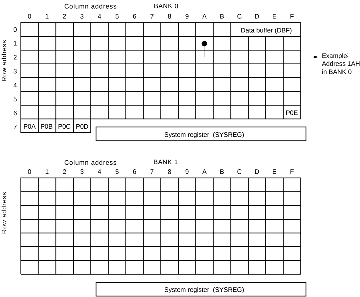
Fig. 2-4 Configuration of Data Memory
