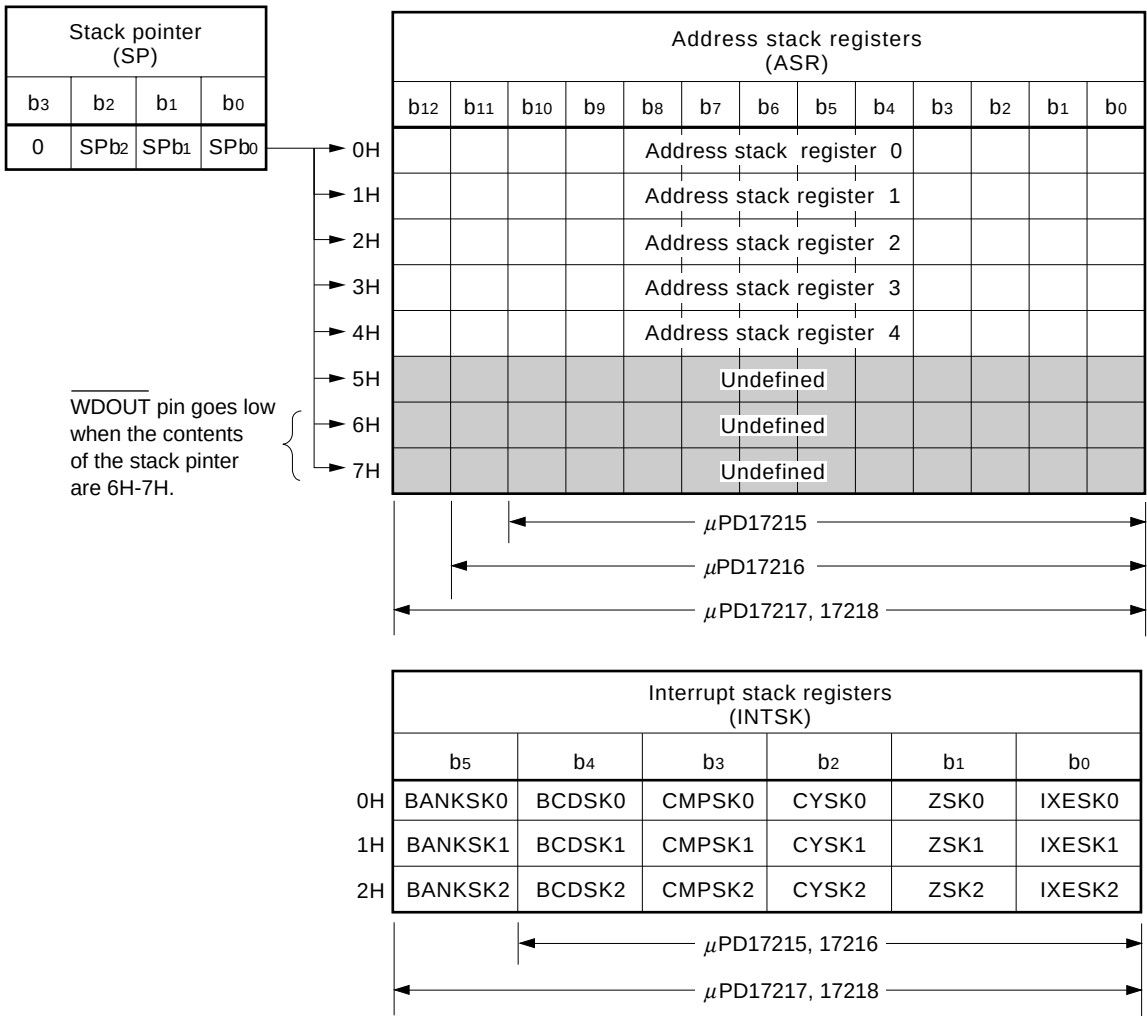
Fig. 2-3 Stack Configuration
