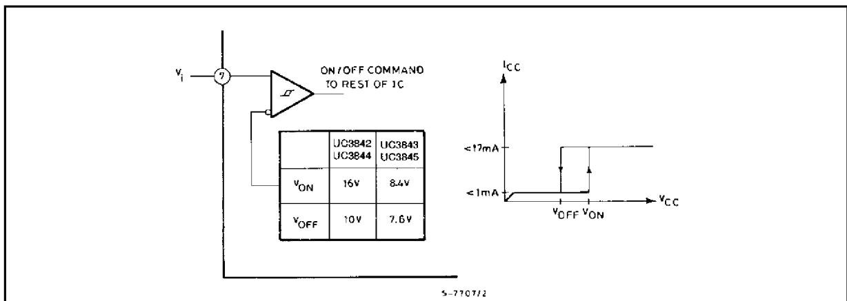
Figure 2 : UnderVoltage Lockout.
