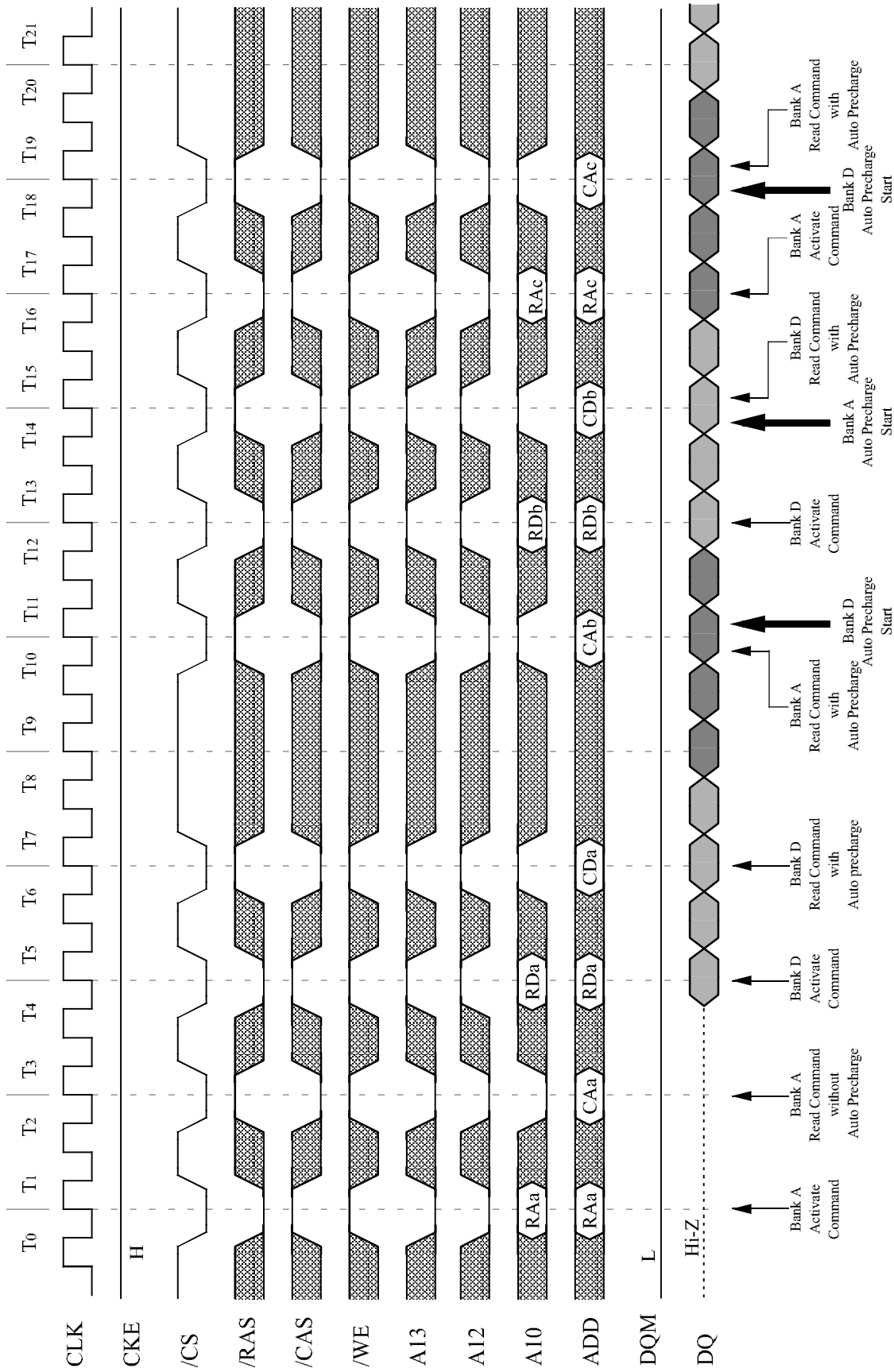
13.19 Auto Precharge after Read Burst (1/2) (Burst length = 4, /CAS latency = 2)
