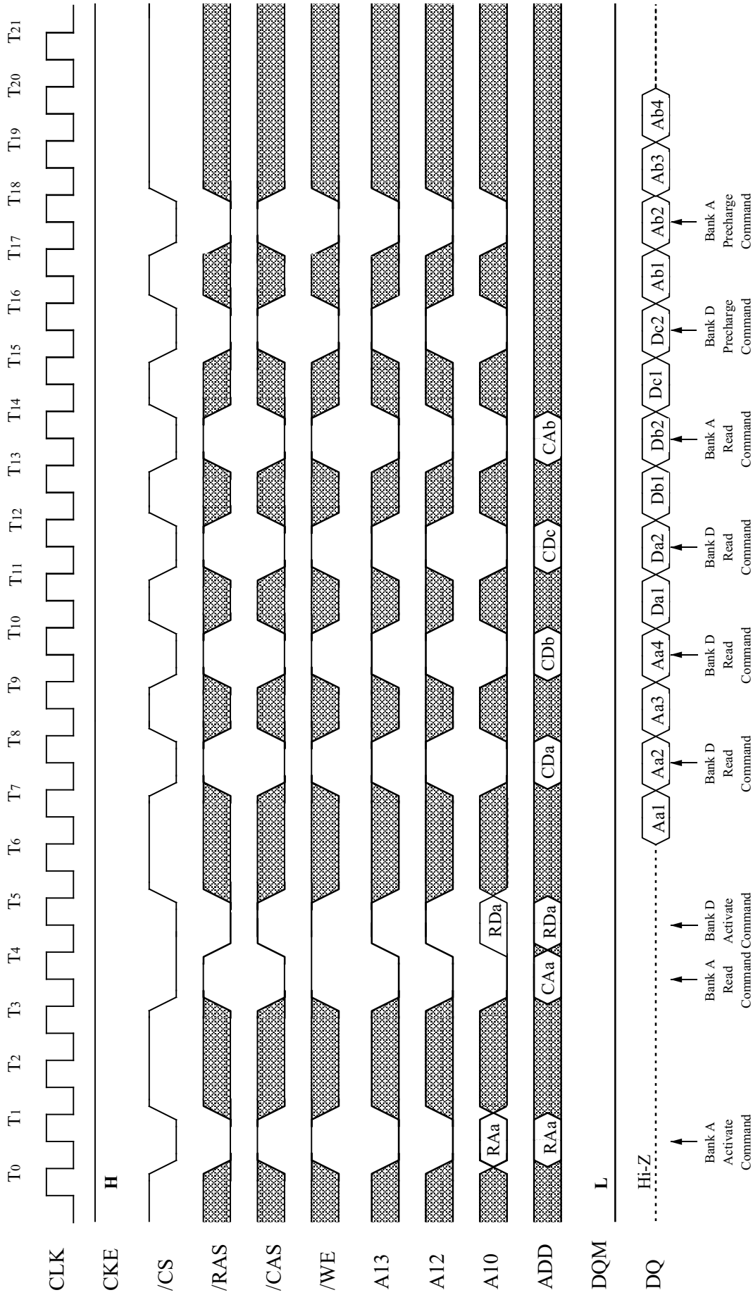
Interleaved Column Read Cycle (2/2) (Burst length = 4, /CAS latency = 3)
