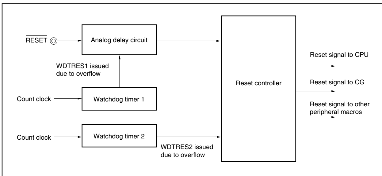
Figure 22-1. Reset Block Diagram
