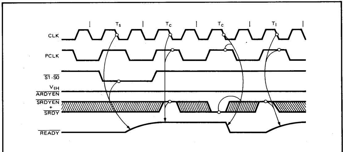
Figure 3. Synchronous Ready Operation
