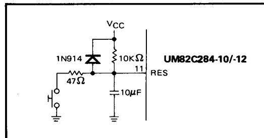
Figure 2. Typical RC \overline{RES} Timing Circuit
