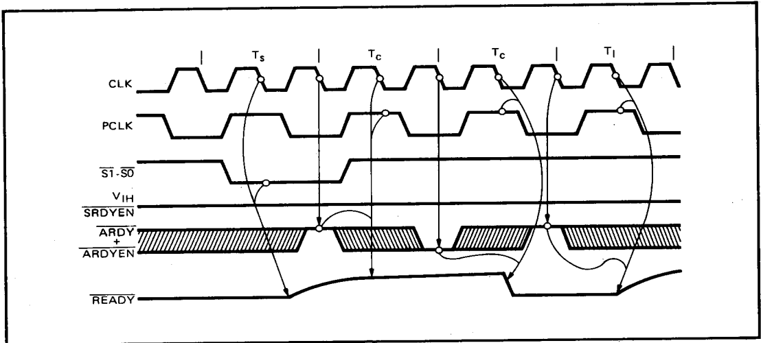
Figure 4. Asynchronous Ready Operation
