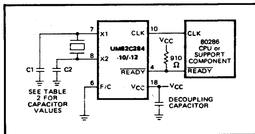
Figure 1. Recommended Crystal and READY Connections
