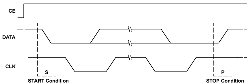
Figure 40. START and STOP Conditions
