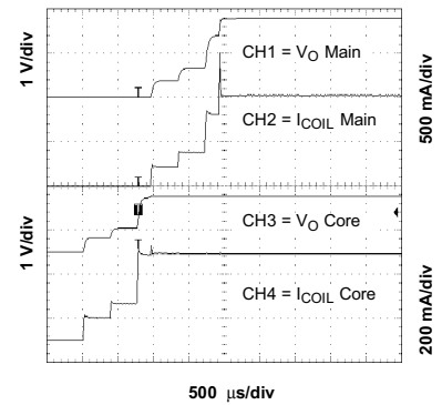
START-UP TIMING
