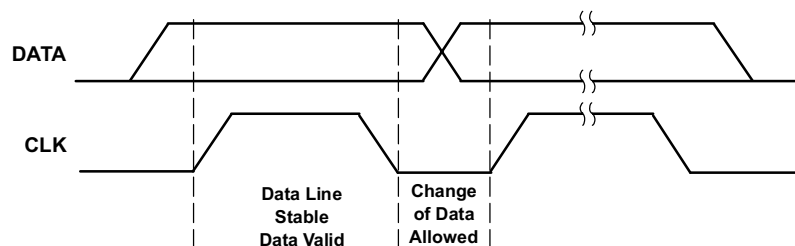
Figure 39. Bit Transfer on the Serial Interface
