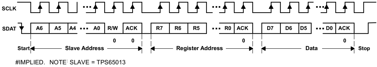
Figure 41. Serial Interface WRITE to TPS65013 Device
