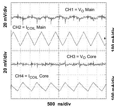
OUTPUT RIPPLE (PWM = 1)
