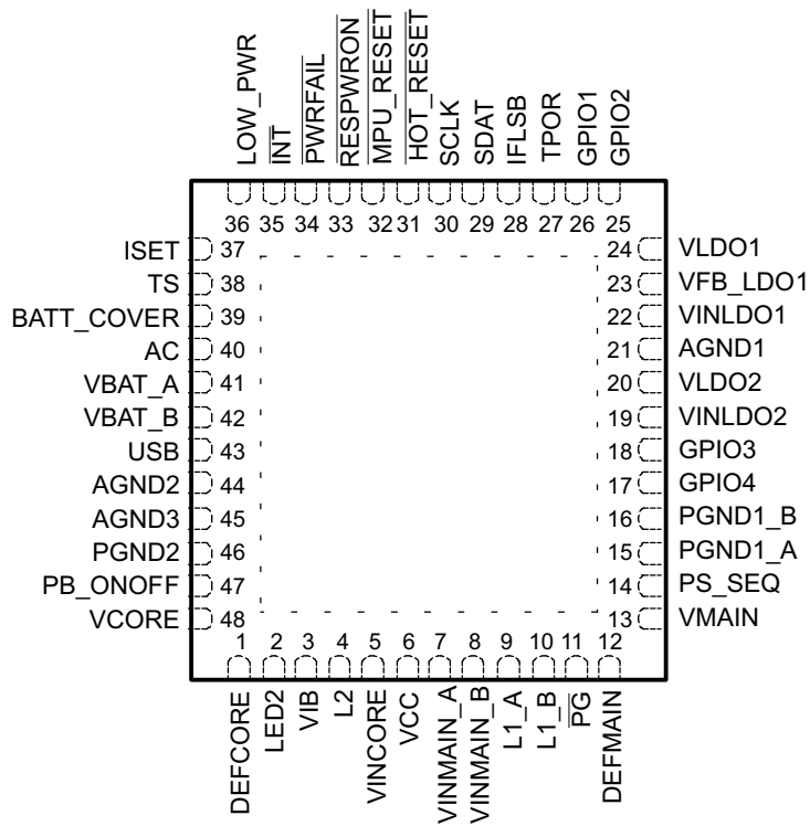
RGZ PACKAGE (TOP VIEW)
