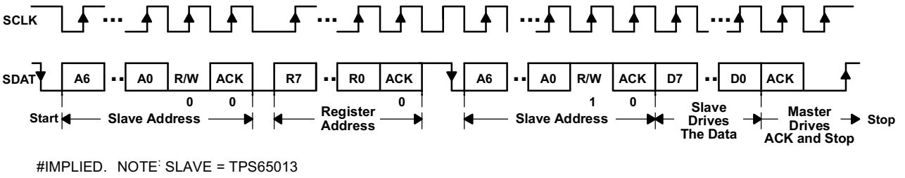
Figure 42. Serial Interface READ From TPS65013: Protocol A
