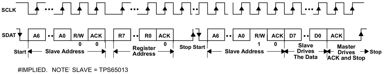
Figure 43. Serial Interface READ From TPS65013: Protocol B
