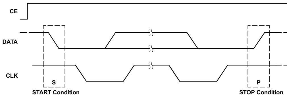
Figure 39. START and STOP Conditions
