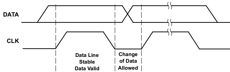
Figure 38. Bit Transfer on the Serial Interface
