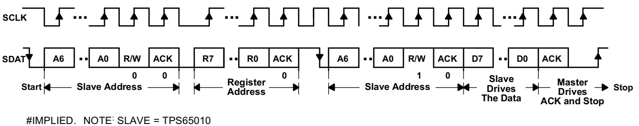
Figure 41. Serial Interface READ From TPS65010: Protocol A
