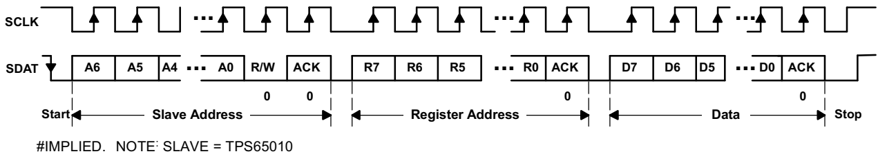
Figure 40. Serial Interface WRITE to TPS65010 Device
