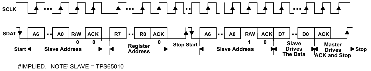
Figure 42. Serial Interface READ From TPS65010: Protocol B
