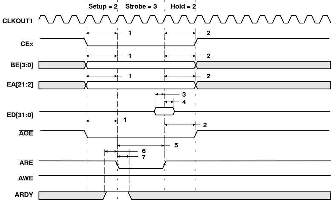
Figure 17. Asynchronous Memory Read Timing (ARDY Not Used)
