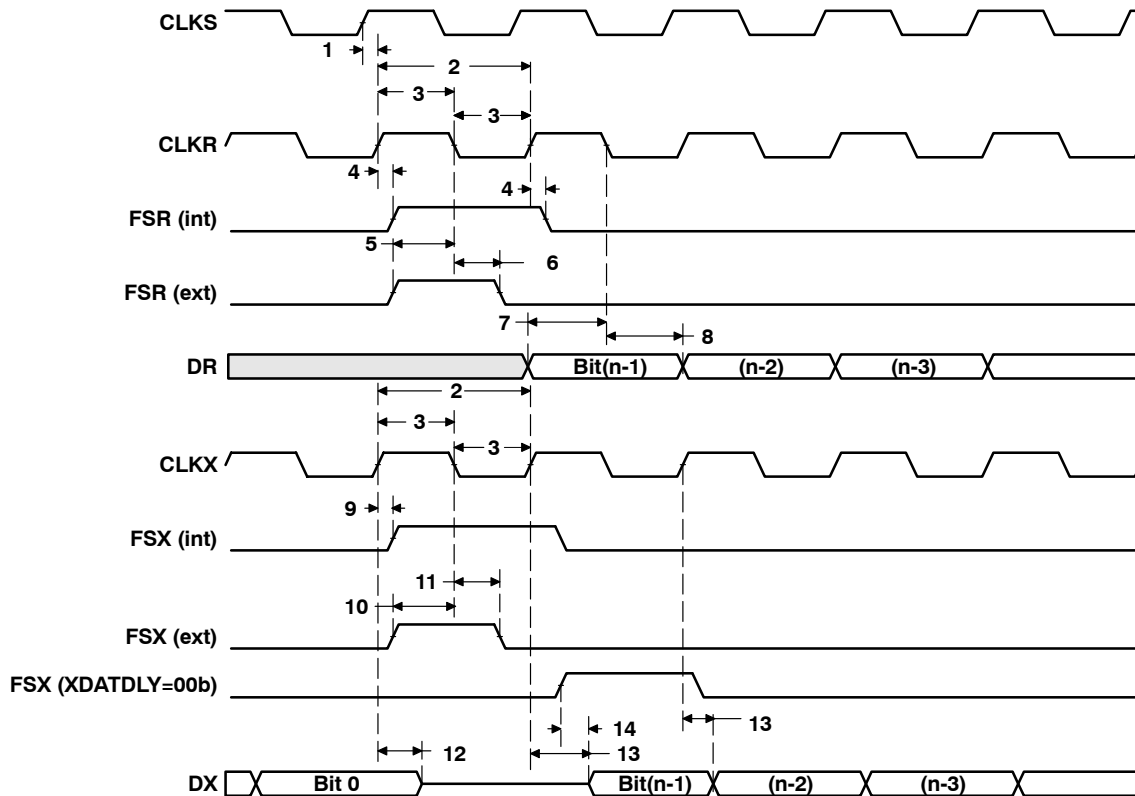
Figure 48. McBSP Timings
