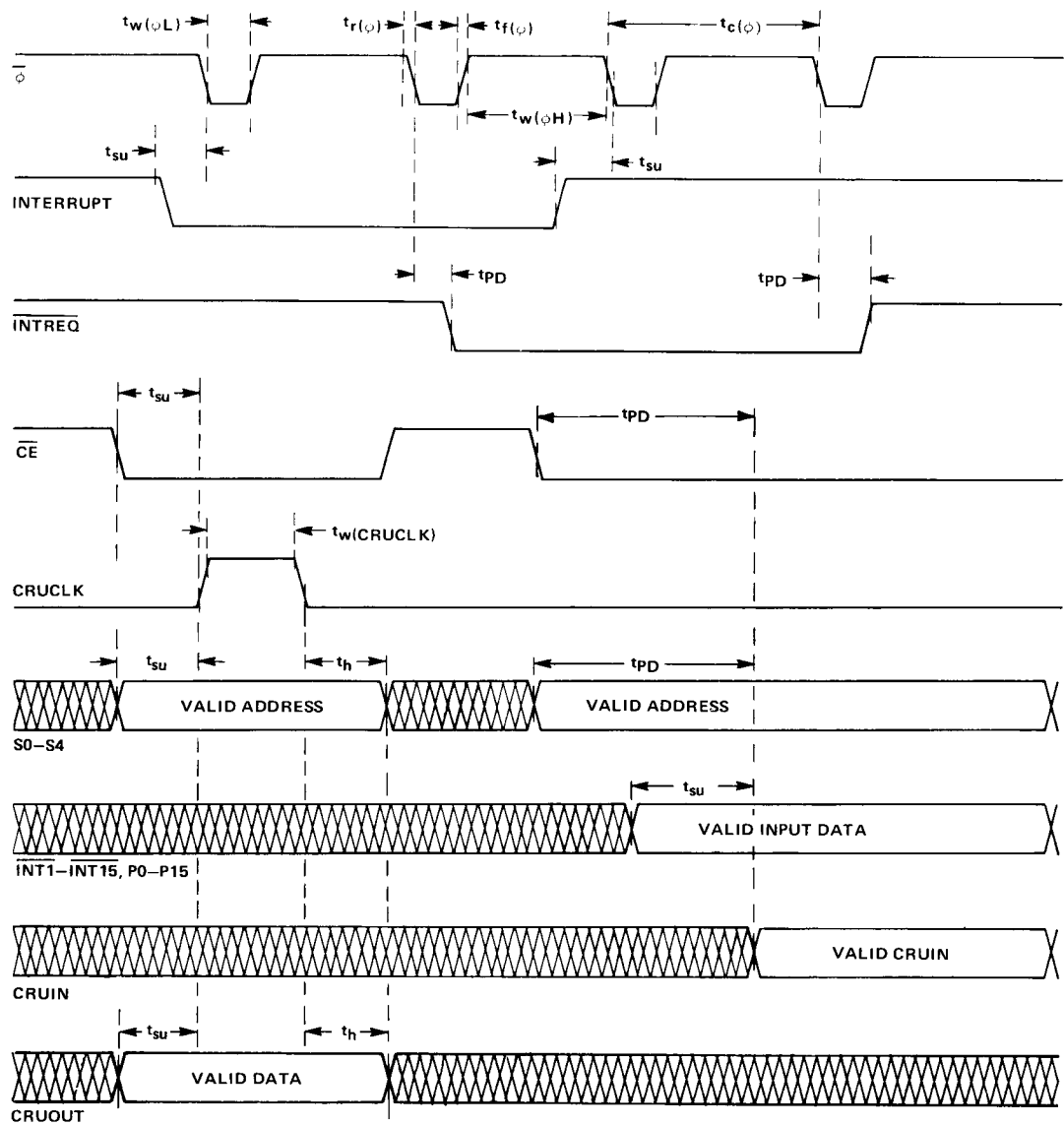
FIGURE 8 – SWITCHING CHARACTERISTICS
