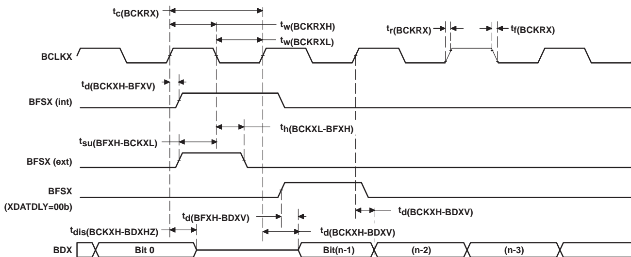
Figure 34. McBSP Transmit Timings
