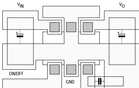
SOT-23L Board Layout
