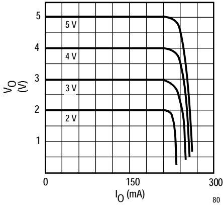
SHORT CURRENT vs. OUTPUT VOLTAGE
