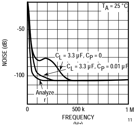
NOISE LEVEL vs. FREQUENCY
