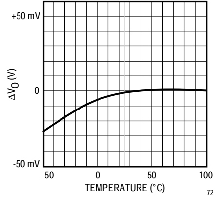
OUTPUT VOLTAGE CHANGE vs. TEMPERATURE
