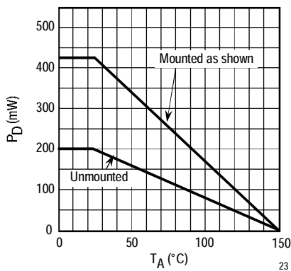
SOT-23L Power Dissipation Curve
