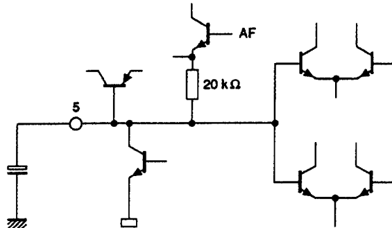
Fig.7 Internal circuits (continued from Fig.6).
