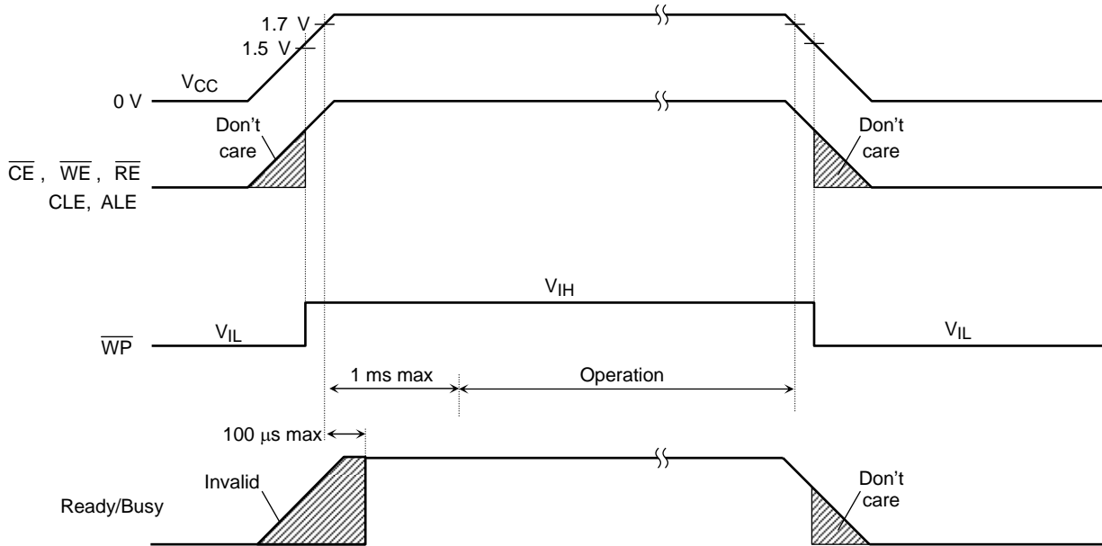
Figure 13. Power-on/off Sequence
