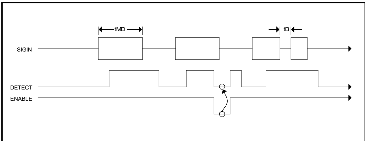
FIGURE 2: Basic Timing
