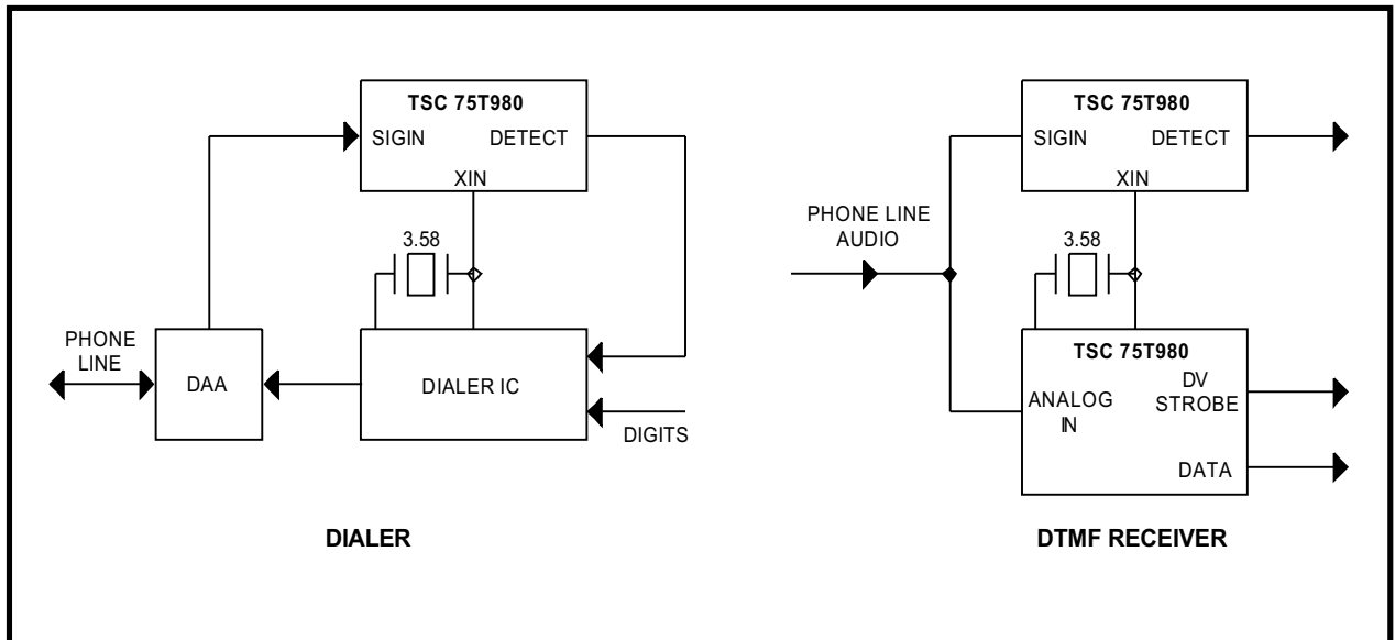
FIGURE 4: Applications Circuits
