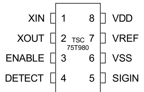
8-Pin DIP
