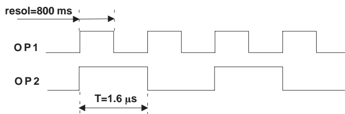
Figure 3. PWM
