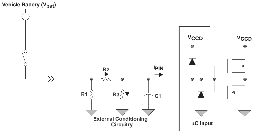
Figure 8. TMS370 Based External Noise Suppression Circuitry
