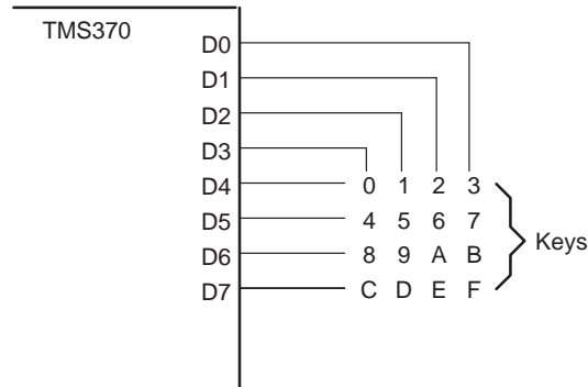
Figure 1. Keyboard Scan Connections to Port D
