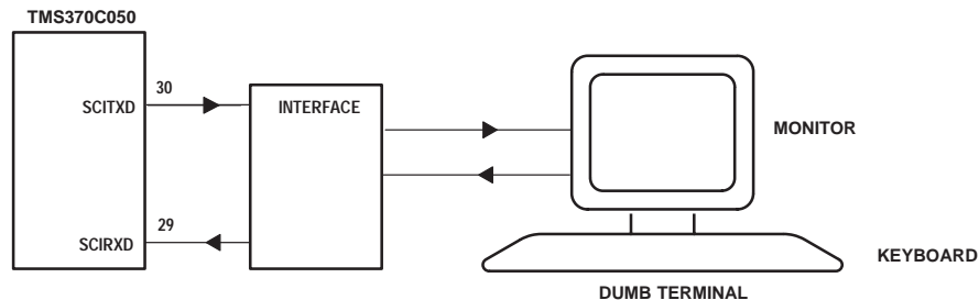
Figure 14. Terminal Interface Example
