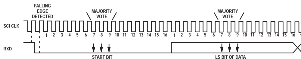
Figure 10. Isosynchronous Communication Format
