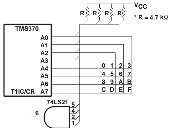
Figure 5. Keyboard Scan Using T1IC/CR as an External Interrupt
