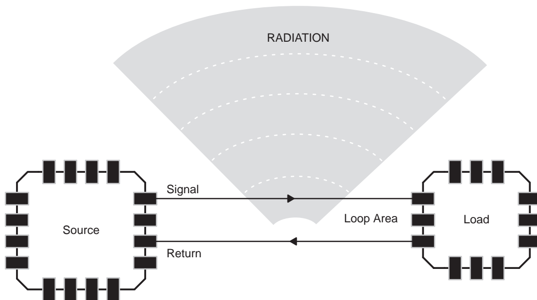
Figure 3. Differential-mode Radiation
