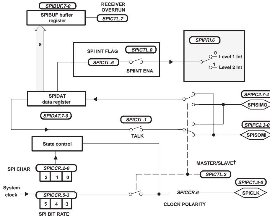
Figure 1. SPI Block Diagram
