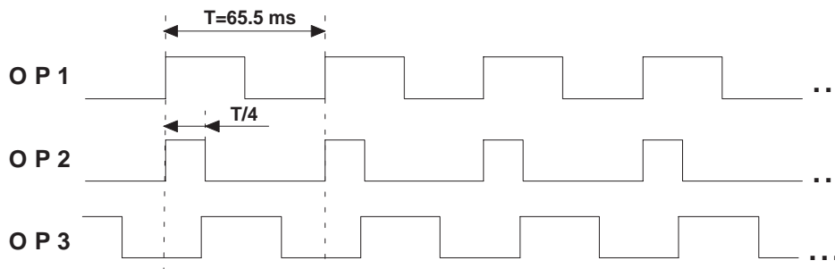
Figure 2. PWM With Period and Duty Cycle Change
