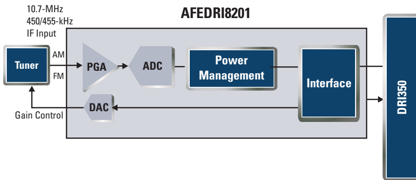
Figure 2. Companion Analog Front End
