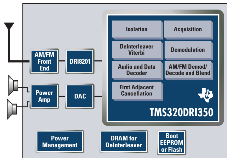
Figure 1. Digital Baseband System
