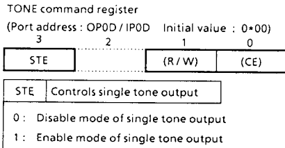
Figure 2. TONE Command Register
