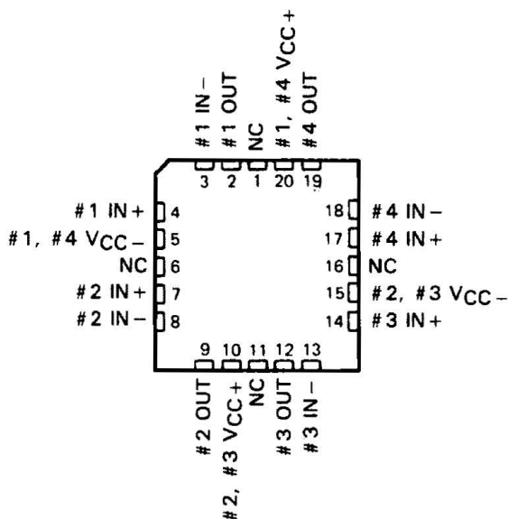
TL044M . . . FK PACKAGE
