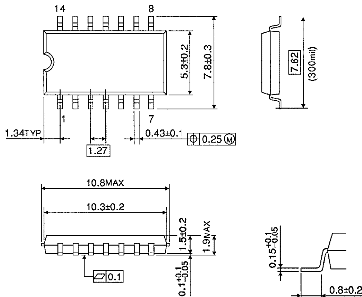
SOP 14PIN (200mil BODY) OUTLINE DRAWING (SOP14-P-300)
