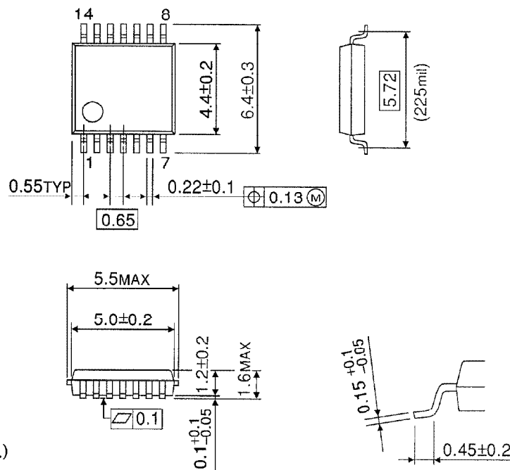
SSOP 14PIN OUTLINE DRAWING (SSOP14-P-225)
