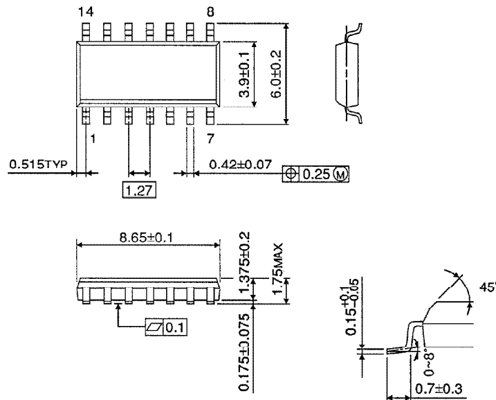
SOP 14PIN (150mil BODY) OUTLINE DRAWING (SOL14-P-150)
