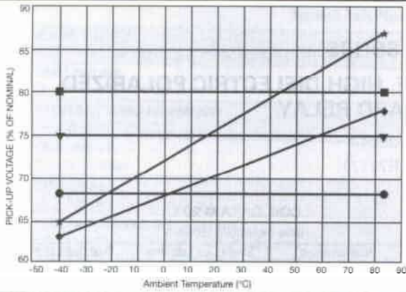
FIGURE 2 - TEMPERATURE VS. PICK-UP VOLTAGE COMPARISON
