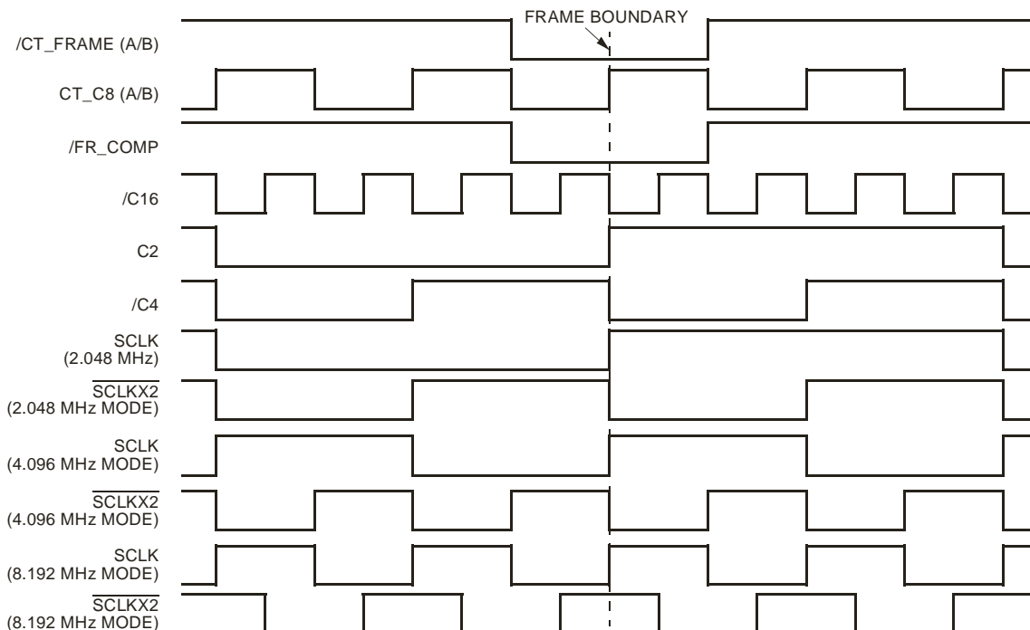
Figure 24. Clock Alignment
