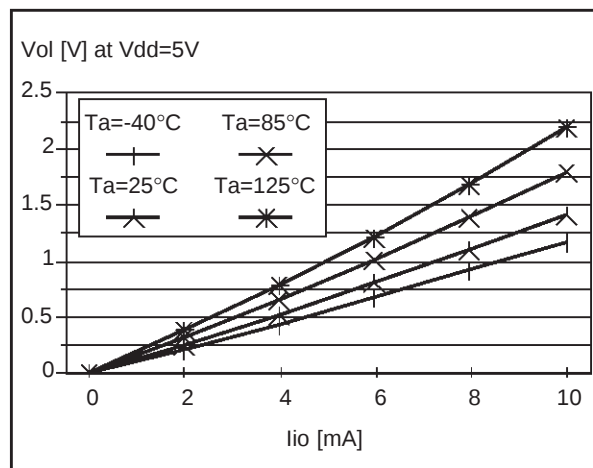
Figure 80. Typical V_{OL} at V_{DD}=5\text{V} (high-sink)
