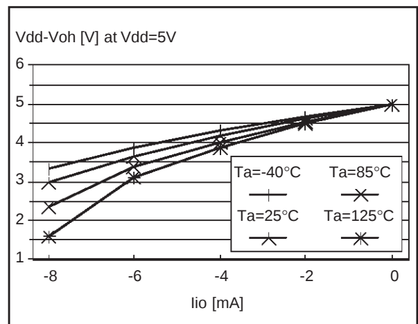
Figure 81. Typical V_{DD}-V_{OH} at V_{DD}=5\text{V}
