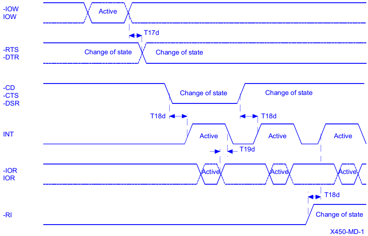
Modem input/output timing
