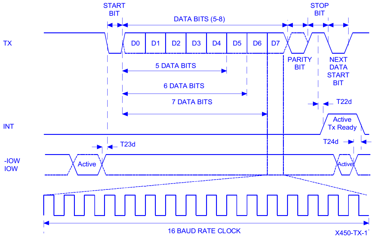
Transmit timing
