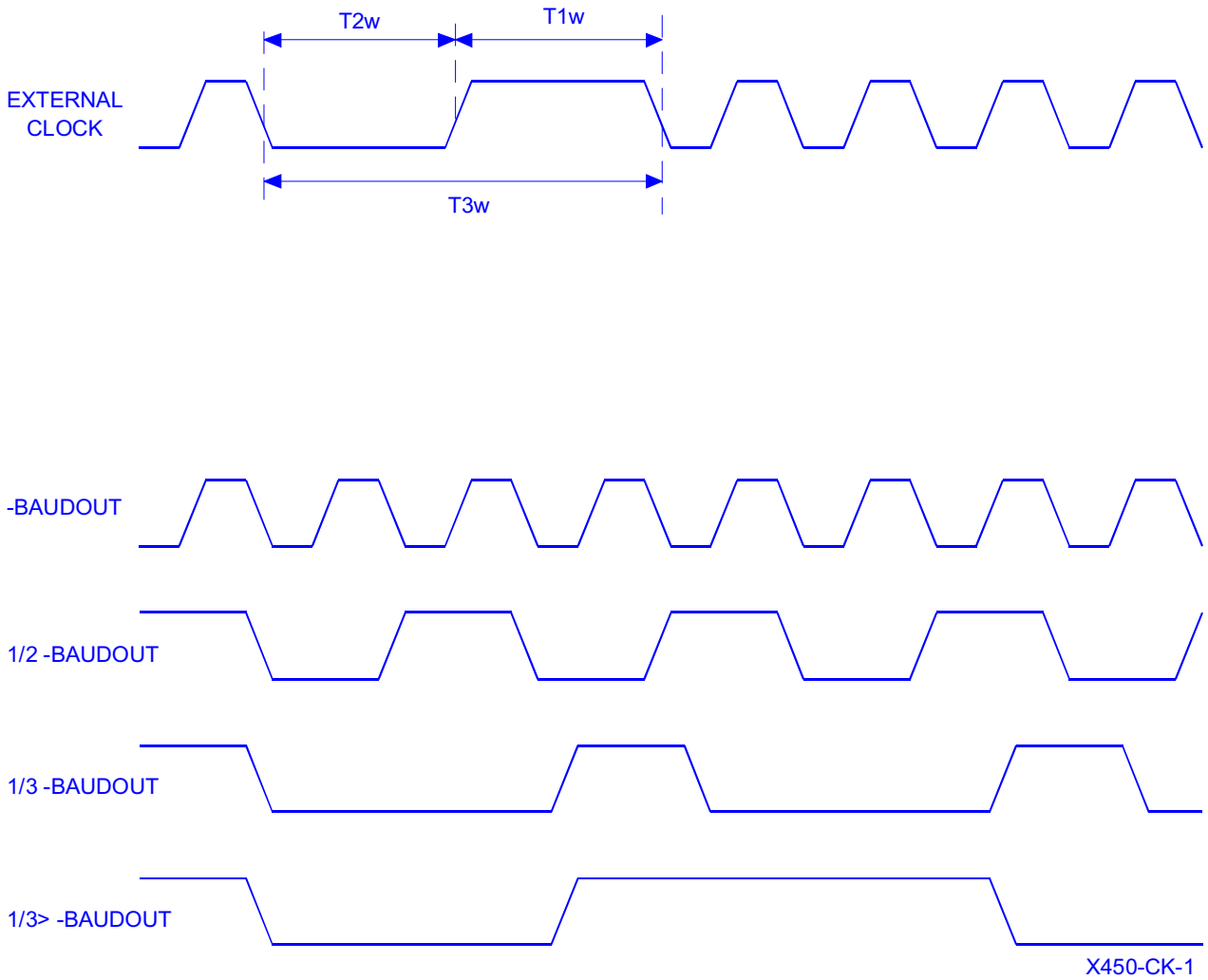
Clock timing
