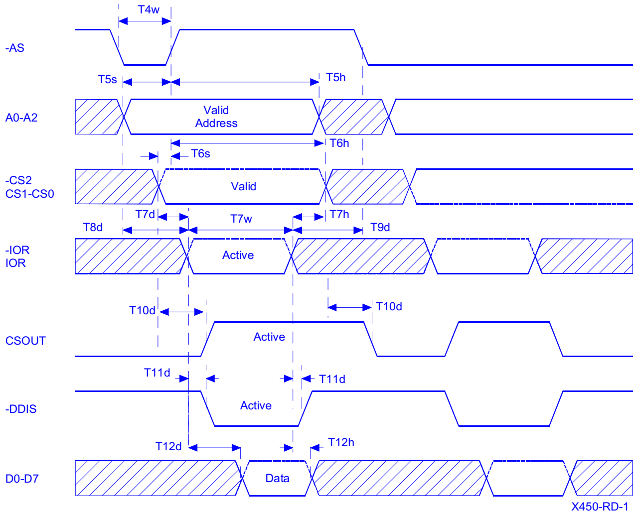
General read timing
