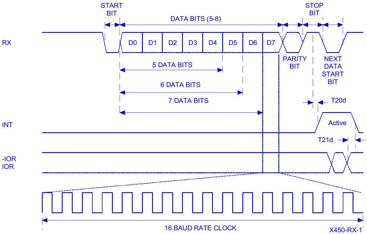
Receive timing
