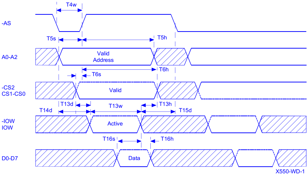
General write timing
