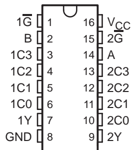
SN54F253 . . . J PACKAGE SN74F253 . . . D OR N PACKAGE (TOP VIEW)
