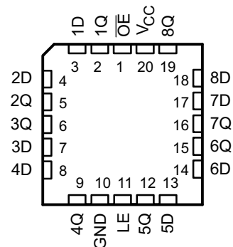
SN54BCT373 . . . FK PACKAGE (TOP VIEW)
