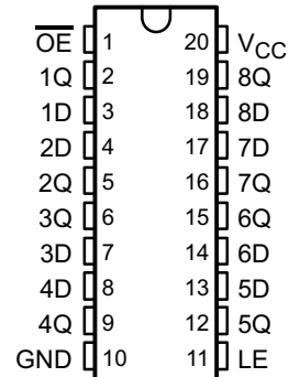
SN54BCT373 . . . J OR W PACKAGE SN74BCT373 . . . DB, DW, OR N PACKAGE (TOP VIEW)
