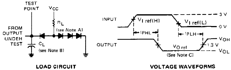
LOAD CIRCUIT
