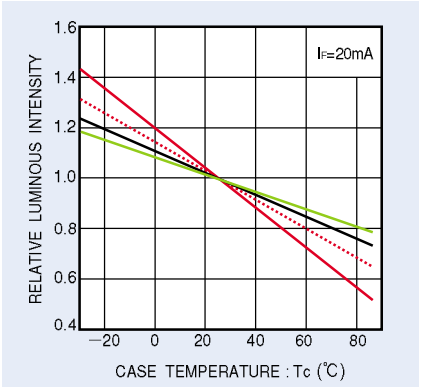
Relative Luminous Intensity - Case Temperature
