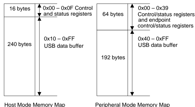
Figure 1. Memory Map
