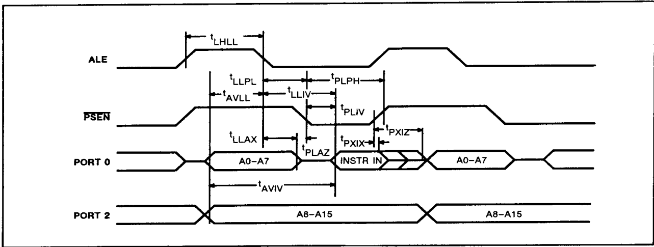
Figure 1. External Program Memory Read Cycle
