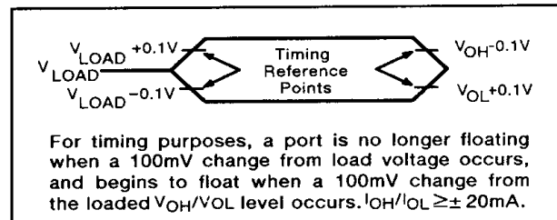
Figure 7. Float Waveform
