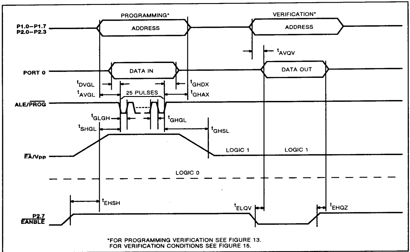
Figure 16. EPROM Programming and Verification
