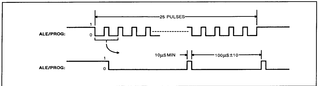
Figure 14. PROG Waveform
