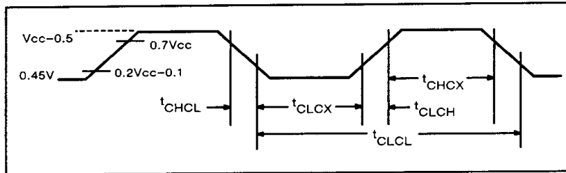
Figure 5. External Clock Drive
