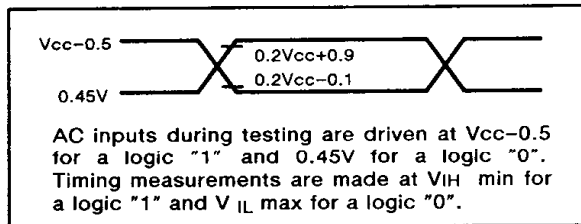
Figure 6. AC Testing Input/Output
