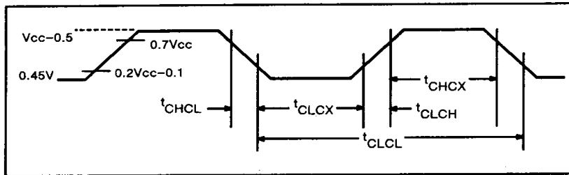
Figure 11. Clock Signal Waveform for I_{CC} Tests in Active and Idle Modes t_{CLCH} = t_{CHCL} = 5ns
