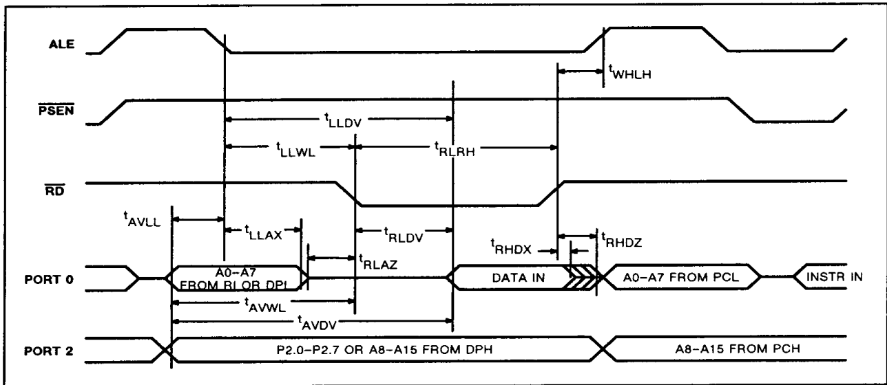
Figure 2. External Data Memory Read Cycle
