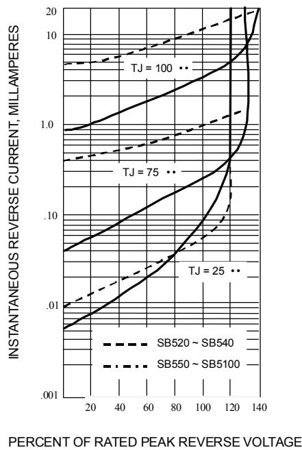
Fig. 3-TYPICAL REVERSE CHARACTERISTICS
