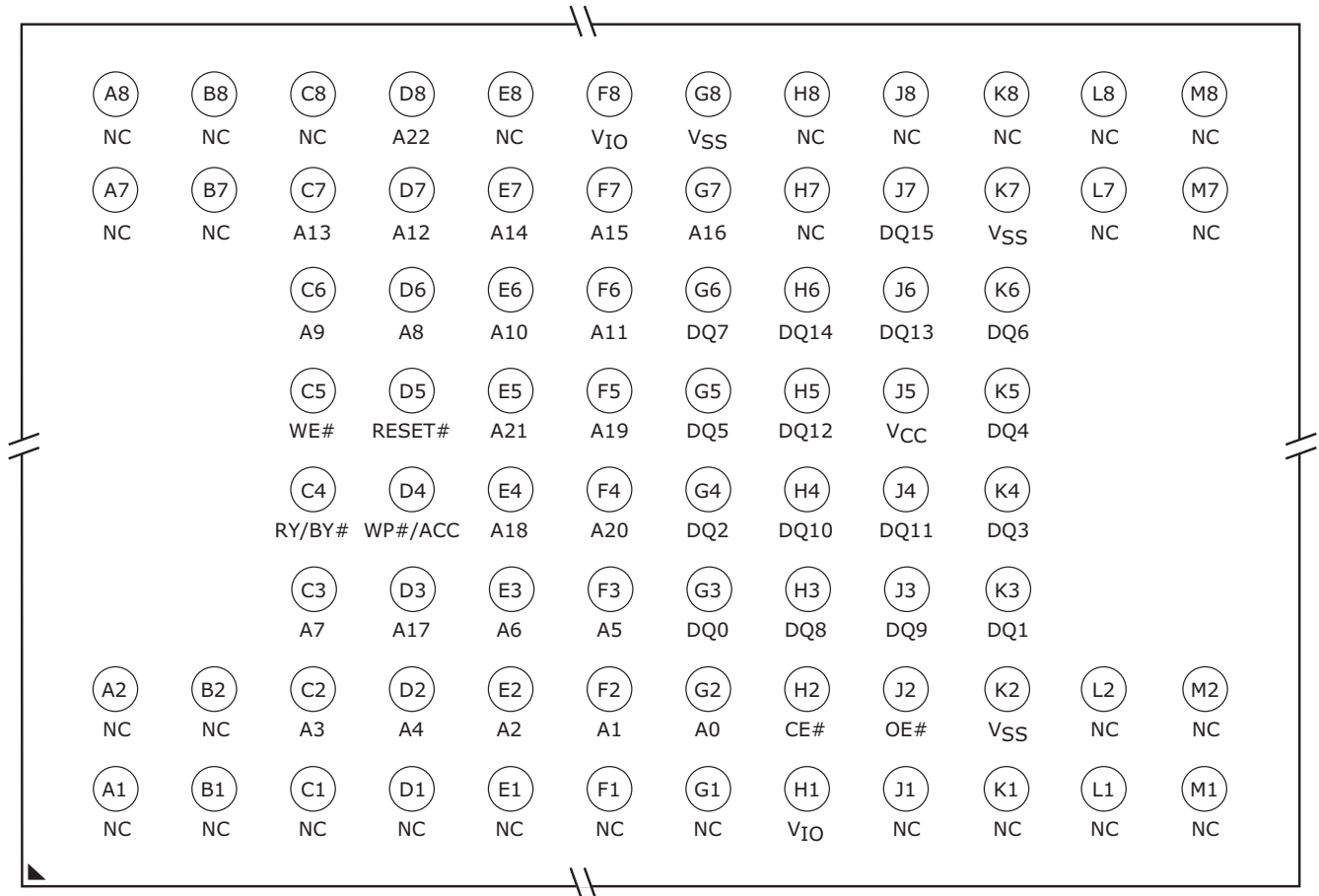
80-Ball Fine-pitch BGA (PL127J) Top View, Balls Facing Down
