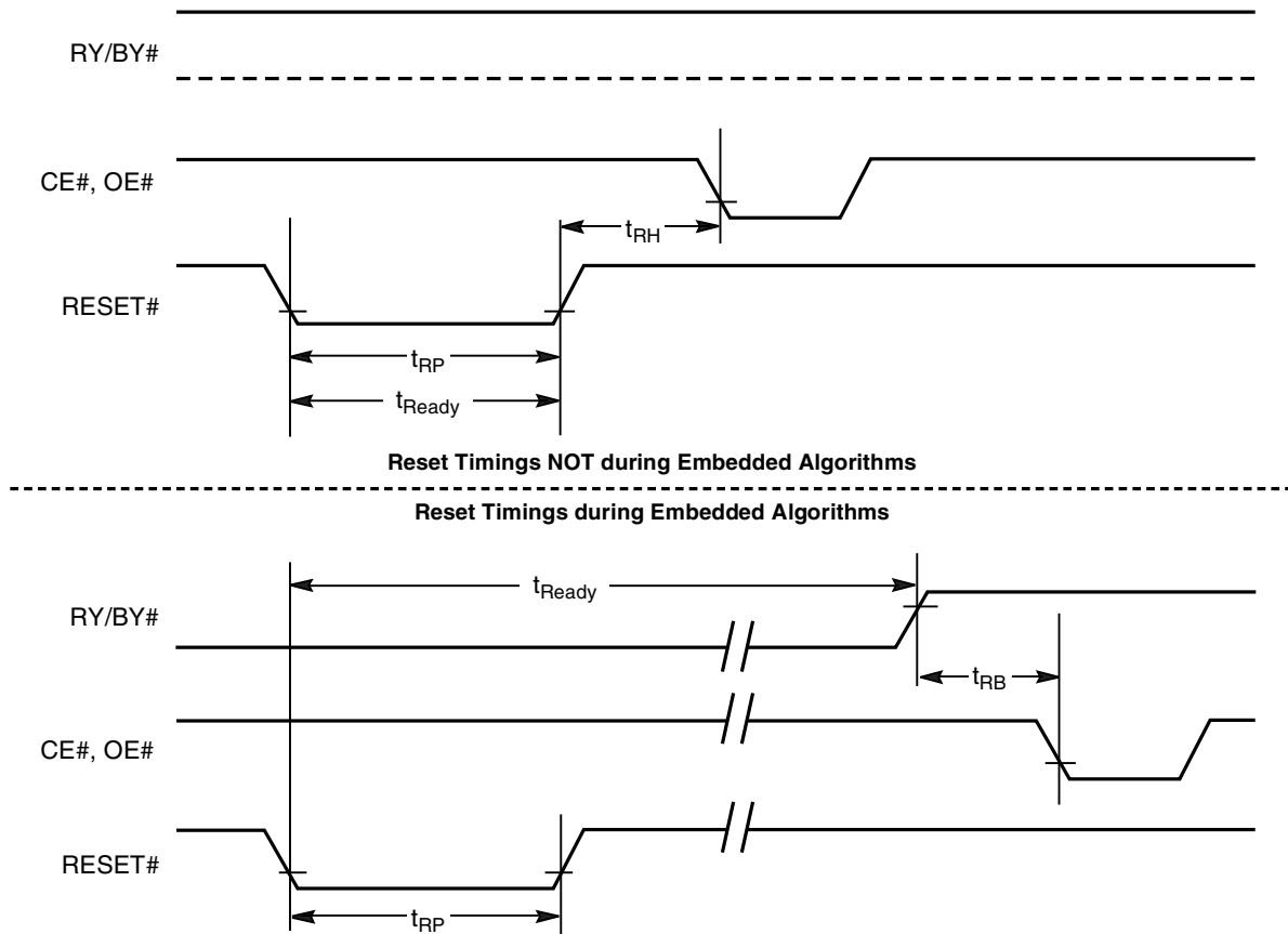
Figure I3. Reset Timings
