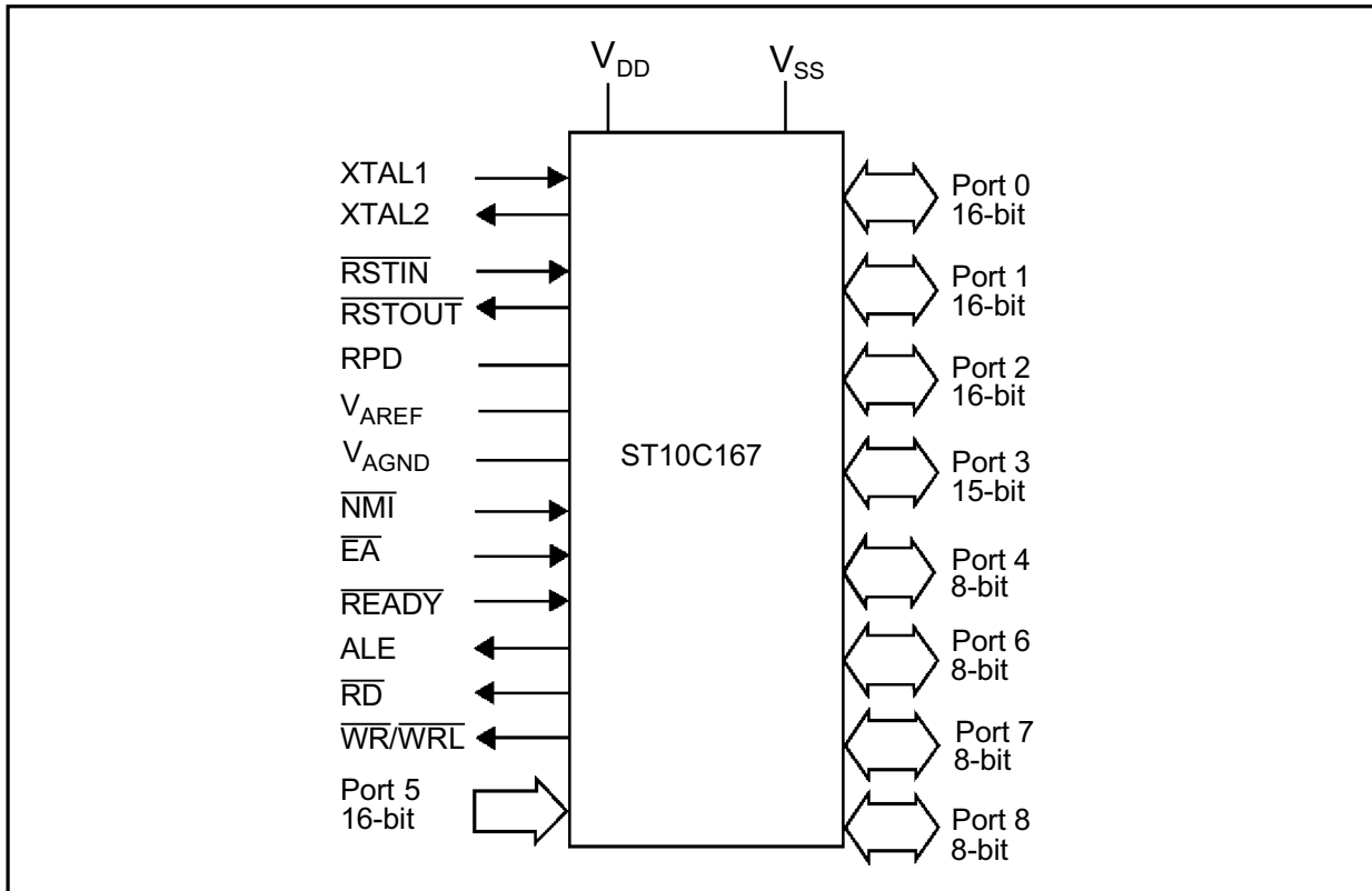
Figure 1 : Logic Symbol
