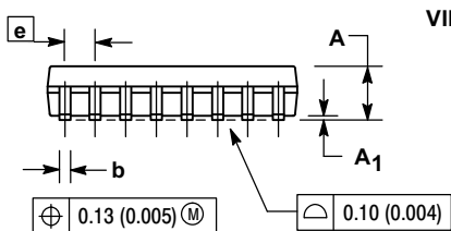
VIEW P
