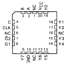
SN54ALS131, SN54AS131A . . . FK PACKAGE (TOP VIEW)
