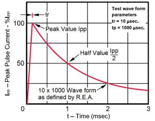
FIGURE 2 – Pulse Waveform
