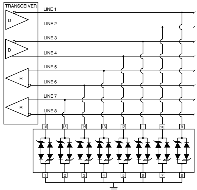
Figure 1. Bidirectional Common-Mode Protection
