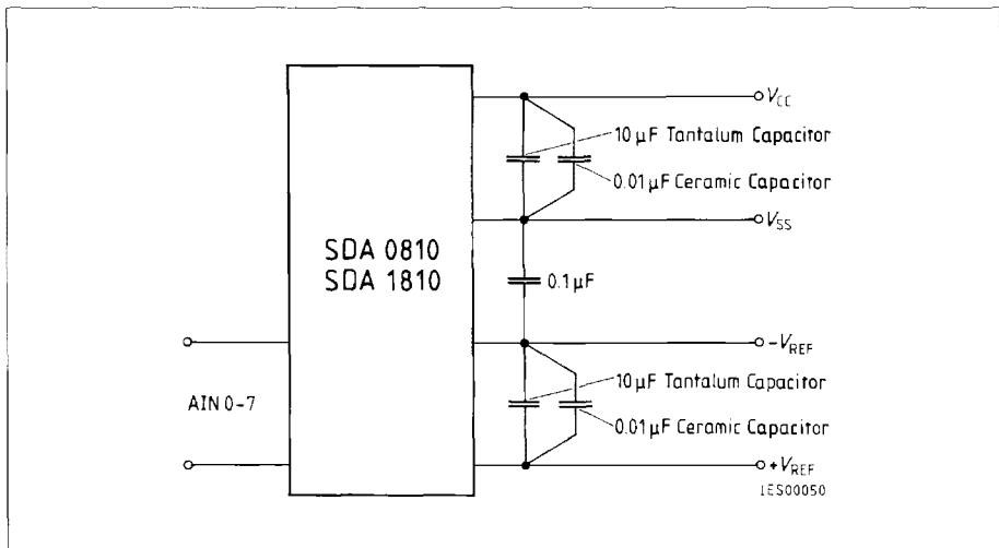
Figure 4 Capacitors
